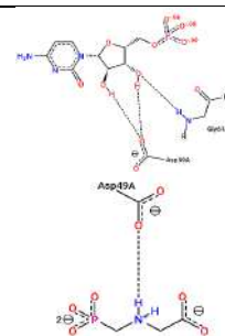
2 possible ligand interactions
