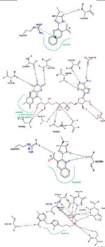
4 possible ligand interactions
