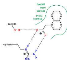
3 possible ligand interactions
