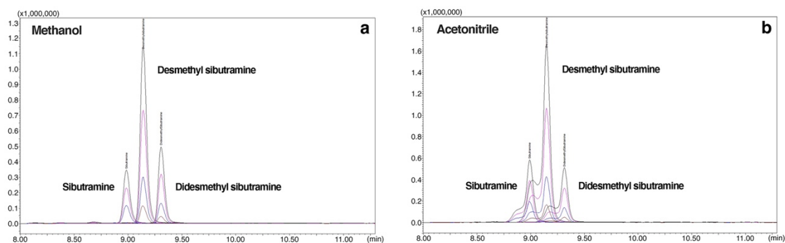
Fig. 2. LC-MS/MS chromatogram of sibutramine, desmethyl sibutramine, and didesmethyl sibutramine after absolute methanol (a) and acetonitrile (b) extraction.
