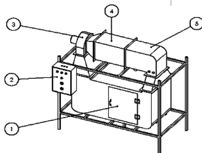
Figure 1 heat pump dryer (1) drying chamber (2) controller (3) blower (4) condenser (5) evaporator
