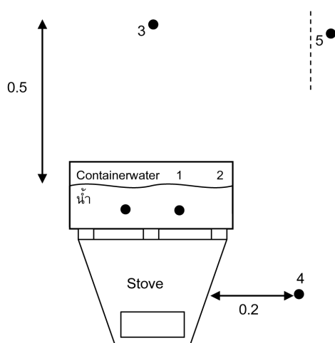
Figure 4 Temperature measurement point
