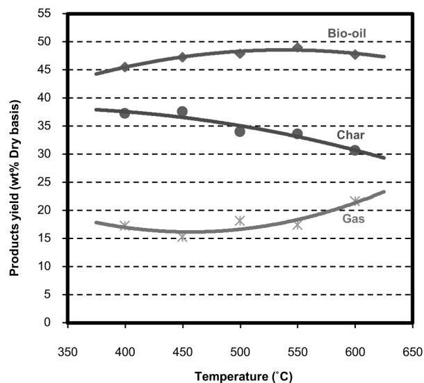
Figure 2 Effect of temperature on products yields
