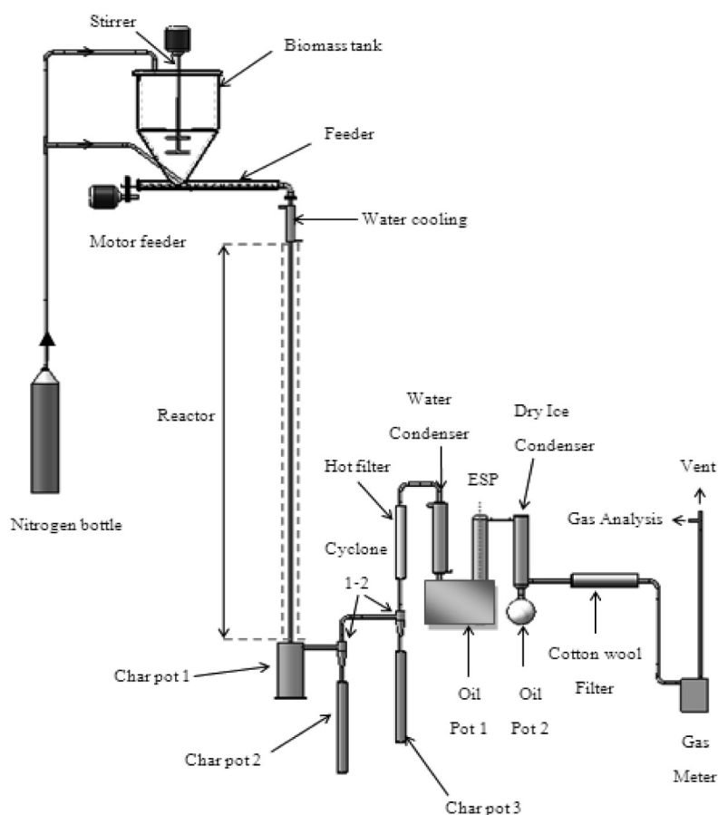
Figure 1 Free-fall pyrolysis reactor unit
