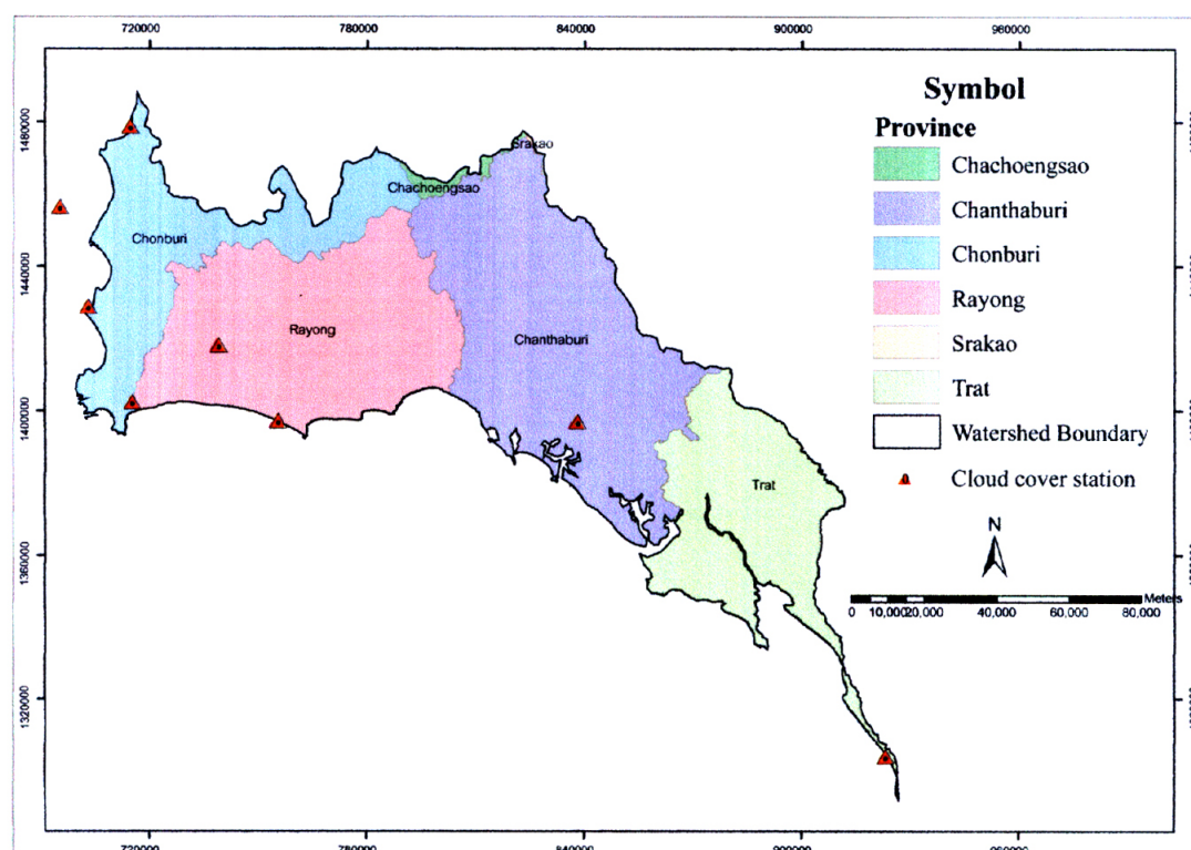
Figure 13 Location of cloudiness stations in this study
