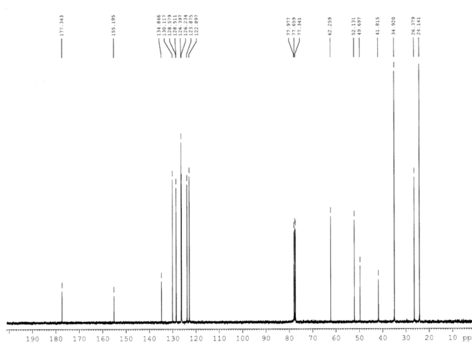
Appendix Figure 2 400 MHz 13 C NMR spectrum of methyl 1-((1-methoxynaphthalen-2-yl)methyl)cyclohexanecarboxylate ( 125 )
