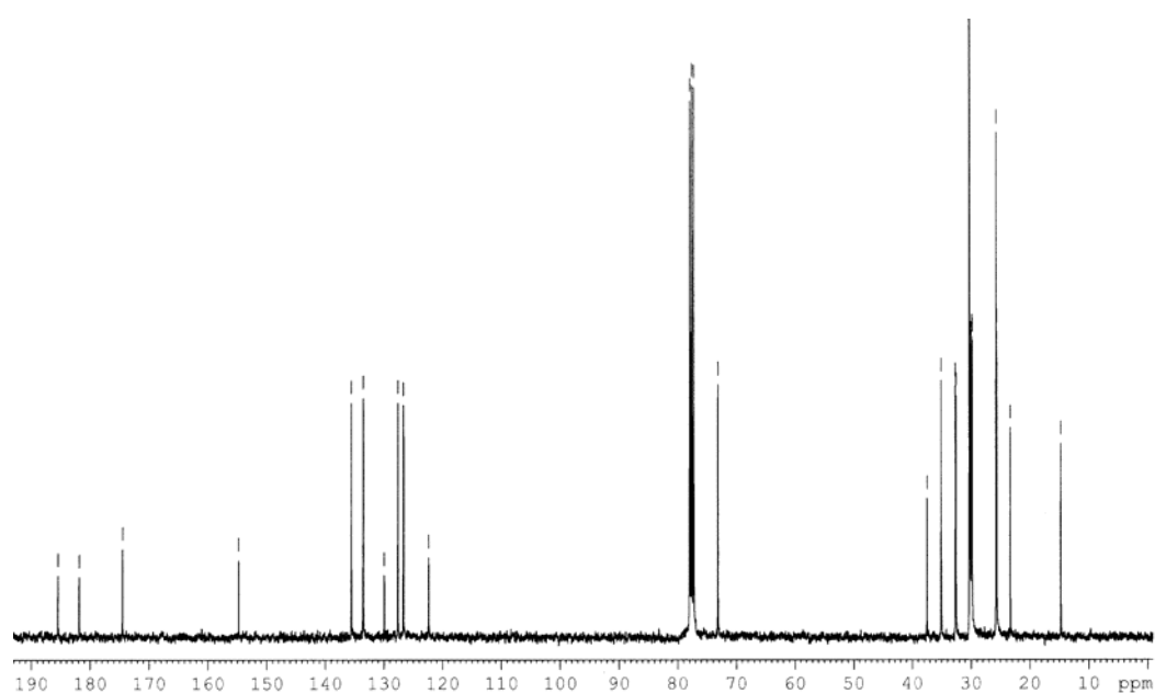
Appendix Figure 44 400 MHz 13 C NMR spectrum of 3-(1,4-dihydro-2-hydroxy-1,4-dioxonaphthalen-3-yl)-2,2-dimethylpropyl tetradecanoate (155)
