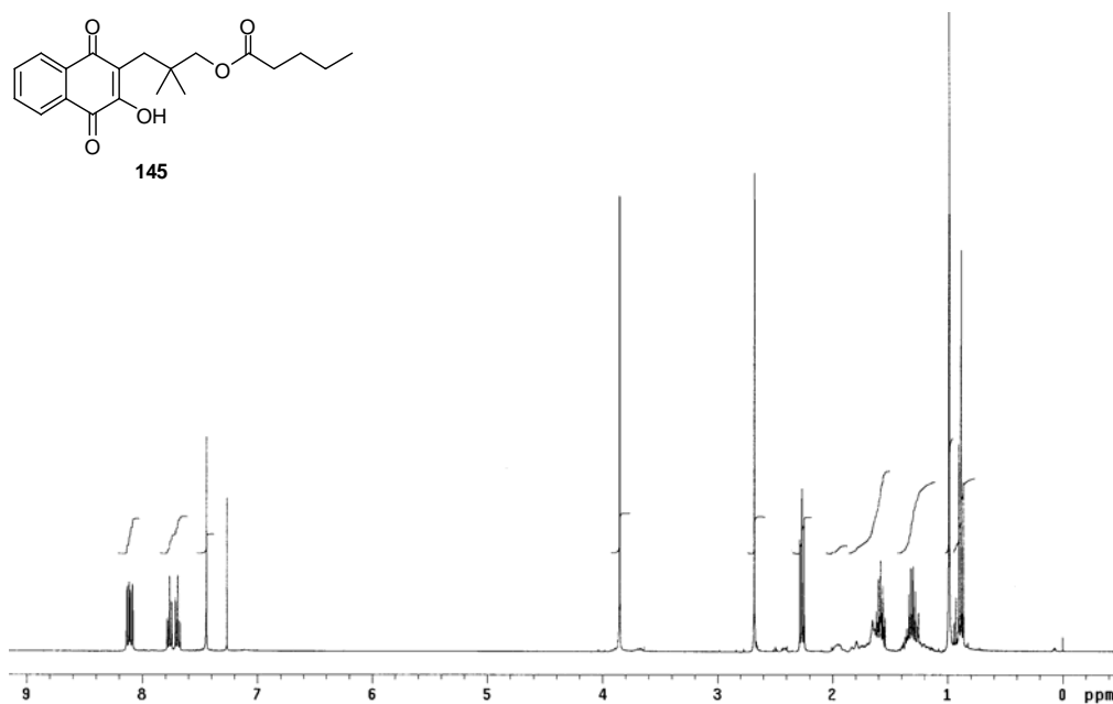
Appendix Figure 23 400 MHz 1 H NMR spectrum of 3-(1,4-dihydro-2-hydroxy-1,4-dioxonaphthalen-3-yl)-2,2-dimethylpropyl pentanoate ( 145 )
