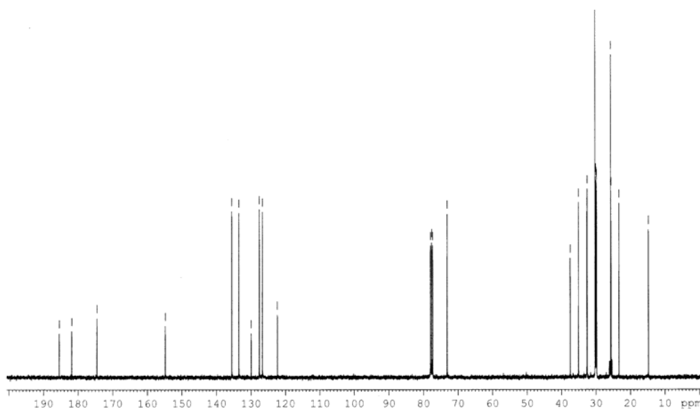
Appendix Figure 42 400 MHz 13 C NMR spectrum of 3-(1,4-dihydro-2-hydroxy-1,4-dioxonaphthalen-3-yl)-2,2-dimethylpropyl dodecanoate ( 154 )
