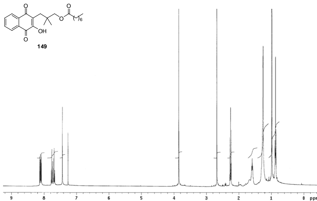
Appendix Figure 31 400 MHz 1 H NMR spectrum of 3-(1,4-dihydro-2-hydroxy-1,4-dioxonaphthalen-3-yl)-2,2-dimethylpropyloctanoate ( 149 )
