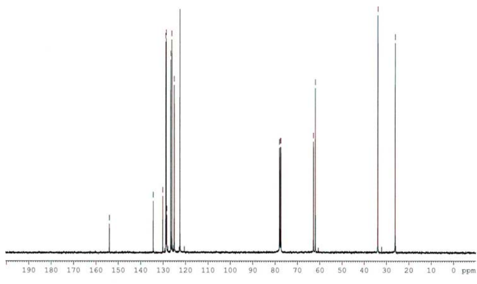
Appendix Figure 68 400 MHz 13 C NMR spectrum of 3-(1-methoxy-naphthalen-2-yl)-propan-1-ol ( 202 )
