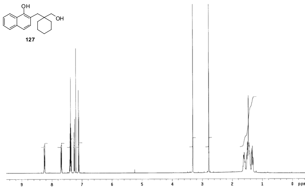
Appendix Figure 5 400 MHz 1 H NMR spectrum of 2-((1-(hydroxymethyl)cyclohexyl)methyl)naphthalen-1-ol ( 127 )
