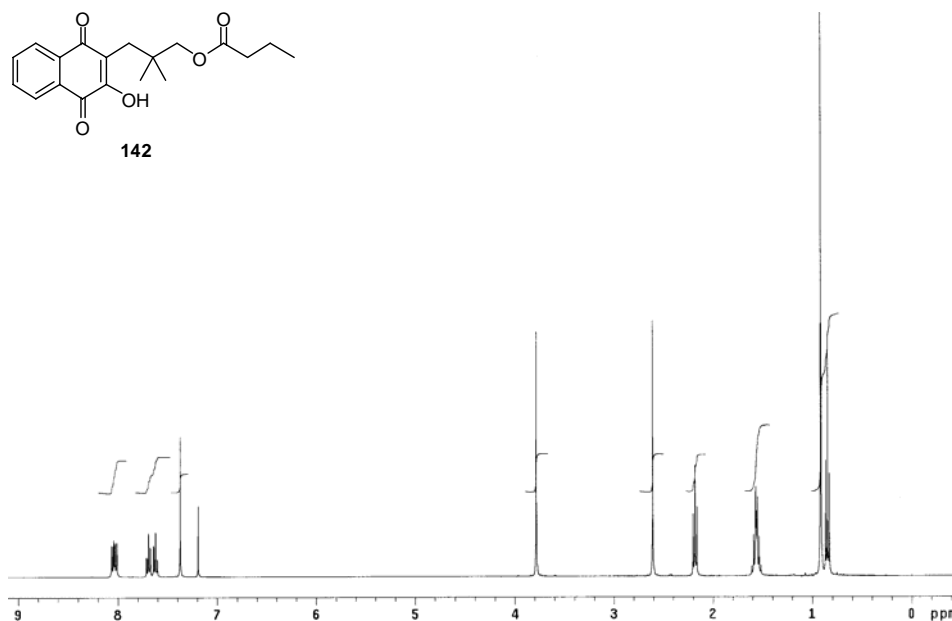
Appendix Figure 17 400 MHz 1 H NMR spectrum of 3-(1,4-dihydro-2-hydroxy-1,4-dioxonaphthalen-3-yl)-2,2-dimethylpropyl butyrate ( 142 )
