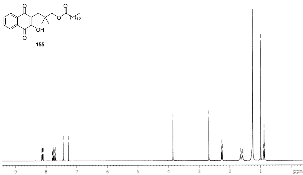
Appendix Figure 43 400 MHz 1 H NMR spectrum of 3-(1,4-dihydro-2-hydroxy-1,4-dioxonaphthalen-3-yl)-2,2-dimethylpropyl tetradecanoate (155)
