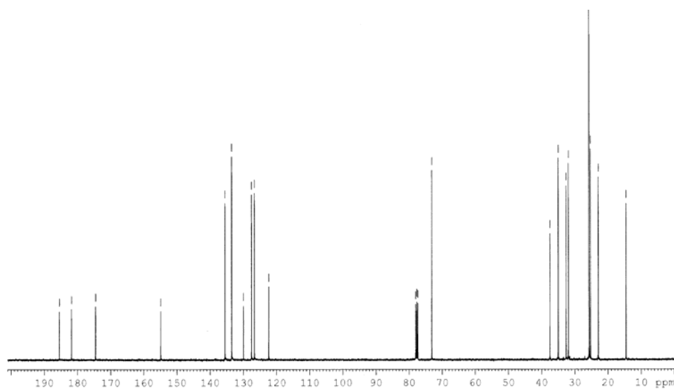
Appendix Figure 24 400 MHz 13 C NMR spectrum of 3-(1,4-dihydro-2-hydroxy-1,4-dioxonaphthalen-3-yl)-2,2-dimethylpropyl pentanoate ( 145 )
