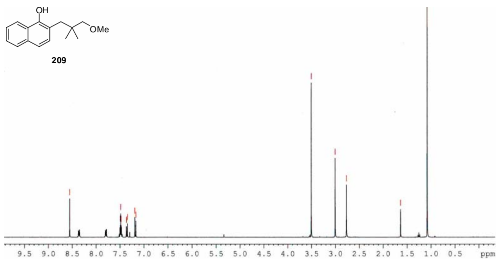
Appendix Figure 81 400 MHz 1 H NMR spectrum of 2-(3-methoxy-2,2-dimethylpropyl)naphthalen-1-ol ( 209 )
