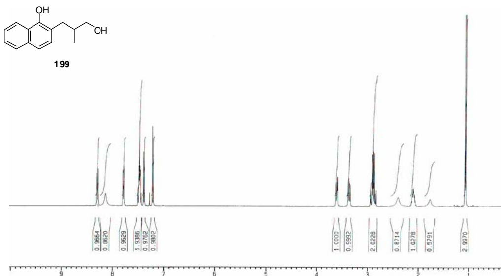
Appendix Figure 63 400 MHz ^1\text{H} NMR spectrum of 2-(3-hydroxy-2-methylpropyl)-naphthalen-1-ol ( 199 )
