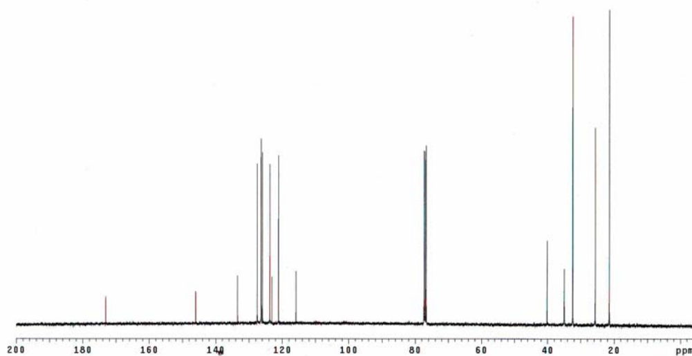
Appendix Figure 4 400 MHz 13 C NMR spectrum of 3,4-dihydro-2-spirocyclohexylbenzo[h]chromen-2-one ( 126 )
