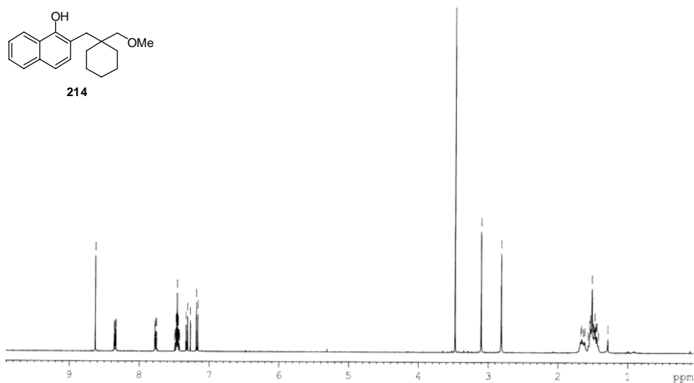
Appendix Figure 91 400 MHz 1 H NMR spectrum of 2-((1-(methoxymethyl)cyclohexyl)methyl)naphthalen-1-ol ( 214 )
