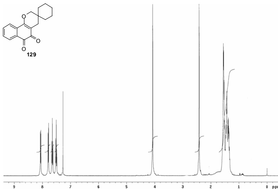
Appendix Figure 9 400 MHz 1 H NMR spectrum of 3,4-dihydro-3,3-spiro cyclohexyl-2H-naphtho[1,2-b]pyran-5,6-dione ( 129 )
