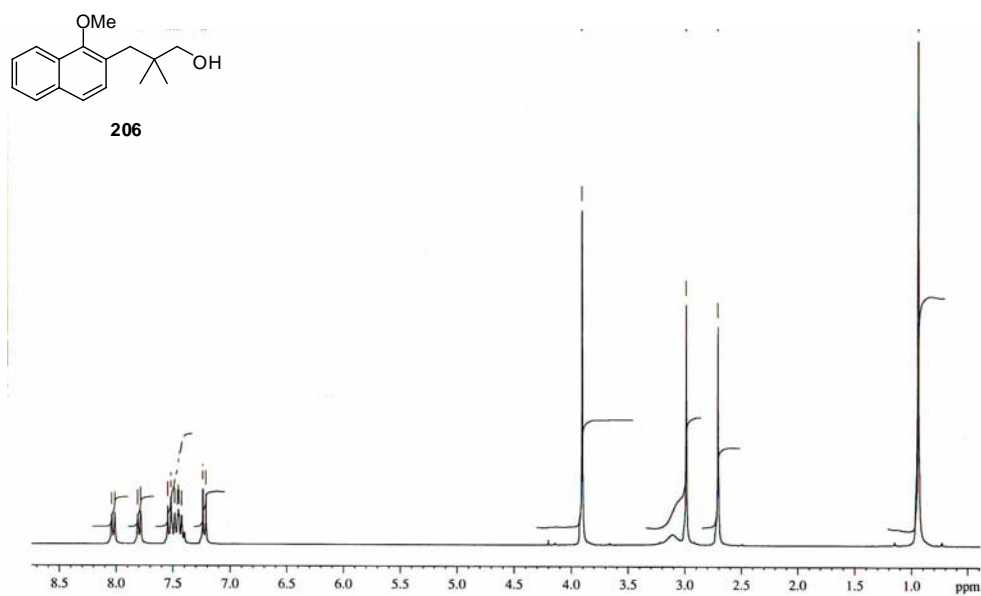
Appendix Figure 75 400 MHz 1 H NMR spectrum of 3-(1-methoxy-naphthalen-2-yl)-2,2-dimethyl-propan-1-ol ( 206 )
