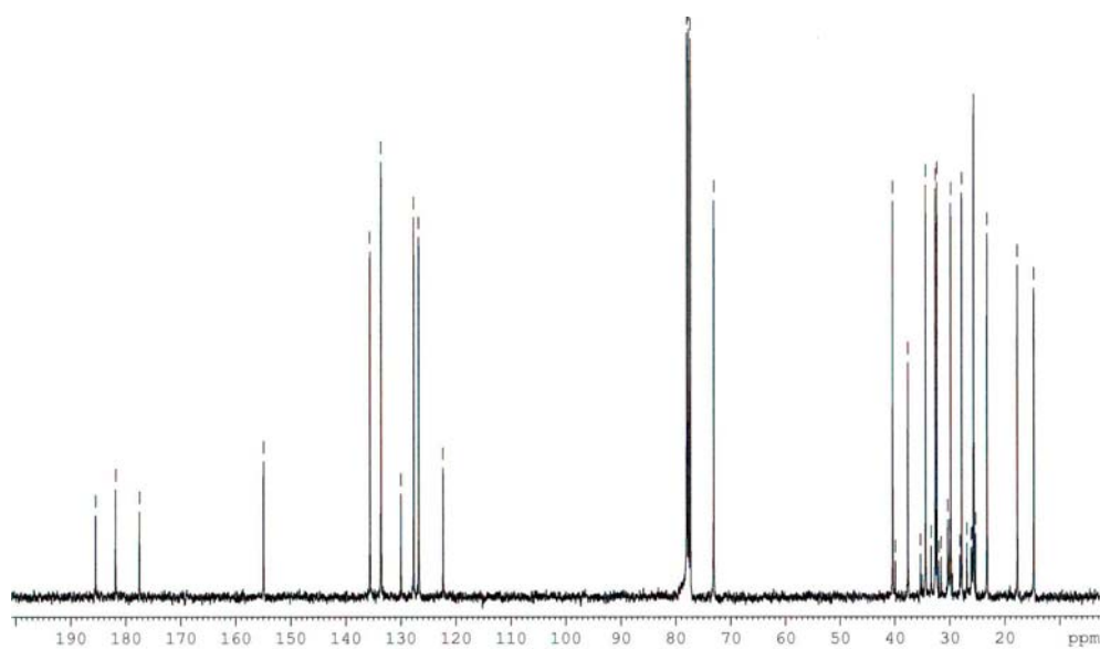
Appendix Figure 34 400 MHz 13 C NMR spectrum of 3-(1,4-dihydro-2-hydroxy-1,4-dioxonaphthalen-3-yl)-2,2-dimethylpropyl 2-methyl octanoate ( 150 )
