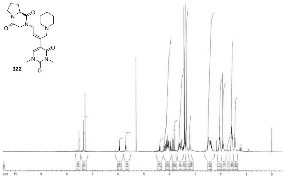
Appendix Figure 105 500 MHz ^{13}\text{C} NMR spectrum of 2-[(2Z)-3-(1,3-dimethyl-2,4-dioxo-1,2,3,4-tetrahydro-pyrimidin-5-yl)-4-piperidin-1-yl-but-2-en-1-yl]-hexahydro-pyrrolo[1,2-a]pyrazine-1,4-dione ( 322 )
