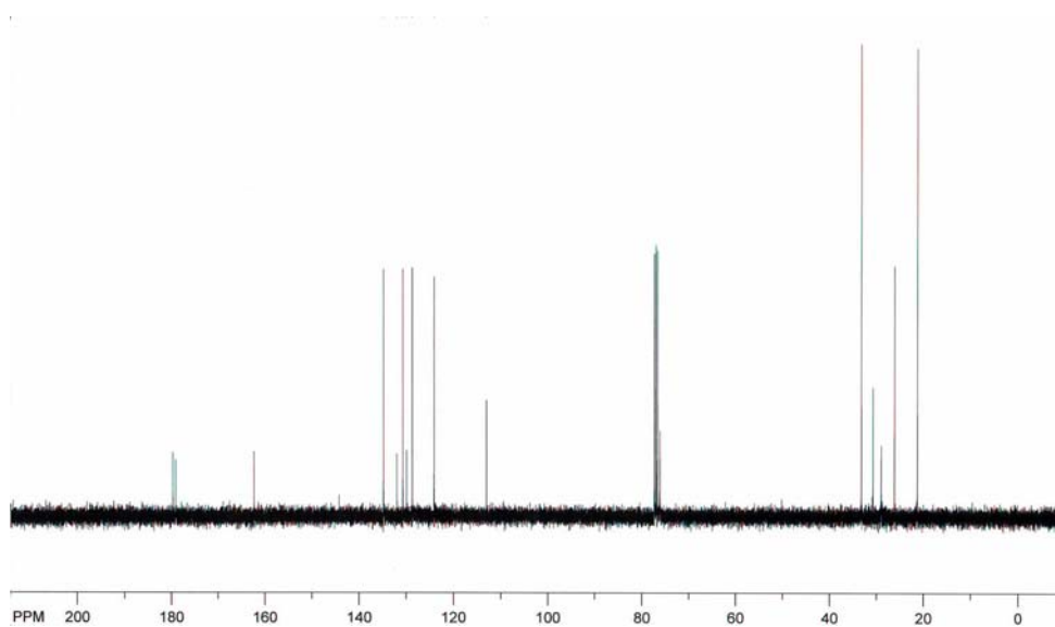
Appendix Figure 10 400 MHz 13 C NMR spectrum of 3,4-dihydro-3,3-spiro cyclohexyl-2H-naphtho[1,2-b]pyran-5,6-dione ( 129 )
