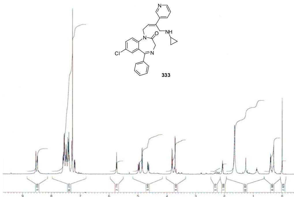
Appendix Figure 116 500 MHz ^{13}\text{C} NMR spectrum of 7-chloro-1-(4-cyclopropylamino-3-pyridin-3-ylbut-2-enyl)-5-phenyl-1,3-dihydrobenzo[e][1,4]diazepin-2-one (333)
