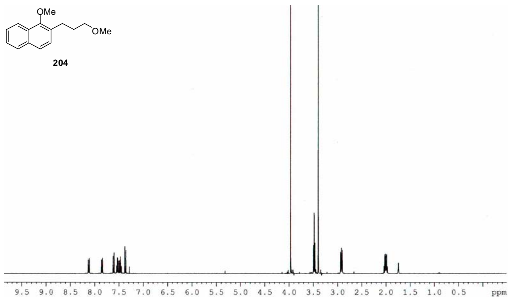
Appendix Figure 71 400 MHz 1 H NMR spectrum of 1-methoxy-2-(3-methoxypropyl)naphthalene ( 204 )
