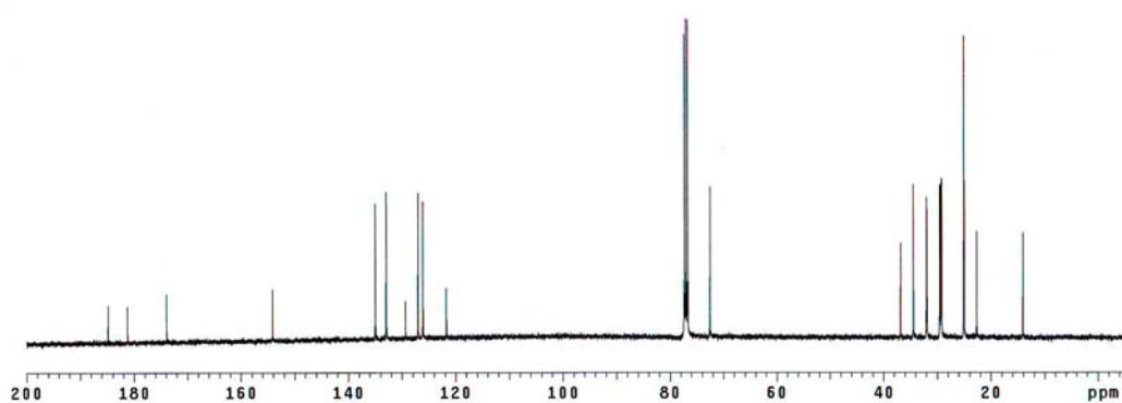
Appendix Figure 40 400 MHz 13 C NMR spectrum of 3-(1,4-dihydro-2-hydroxy-1,4-dioxonaphthalen-3-yl)-2,2-dimethylpropyl undecanoate ( 153 )
