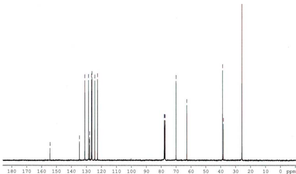
Appendix Figure 76 400 MHz 13 C NMR spectrum of 3-(1-methoxy-naphthalen-2-yl)-2,2-dimethyl-propan-1-ol ( 206 )
