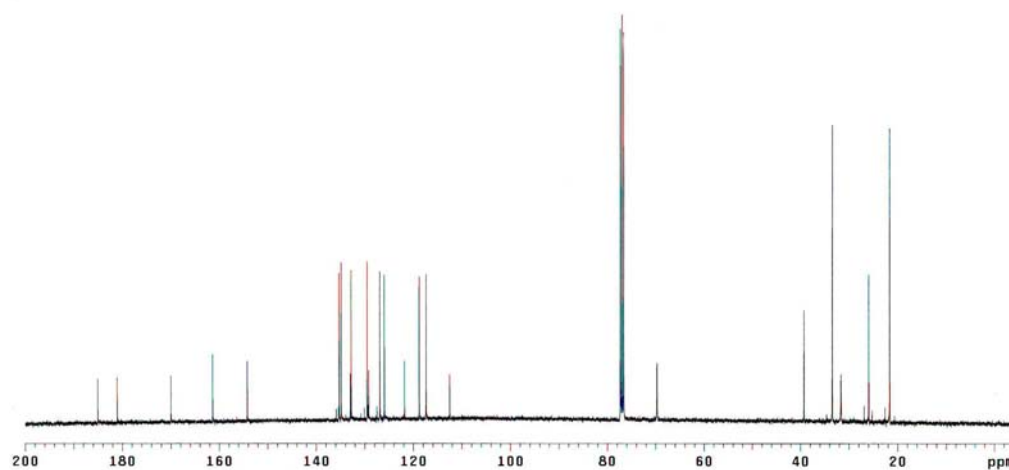
Appendix Figure 58 400 MHz 13 C NMR spectrum of (1-((1,4-dihydro-2-hydroxy-1,4-dioxonaphthalen-3-yl)methyl)cyclohexyl)methyl 2-hydroxybenzoate ( 163 )
