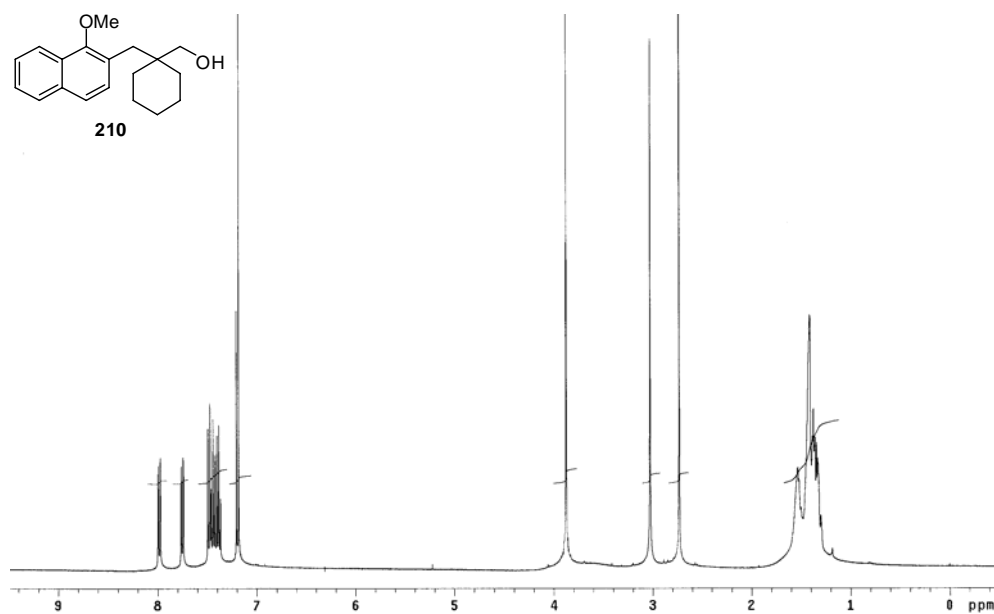
Appendix Figure 83 400 MHz 1 H NMR spectrum of (1-((1-methoxynaphthalen-2-yl)methyl)cyclohexyl)methanol ( 210 )
