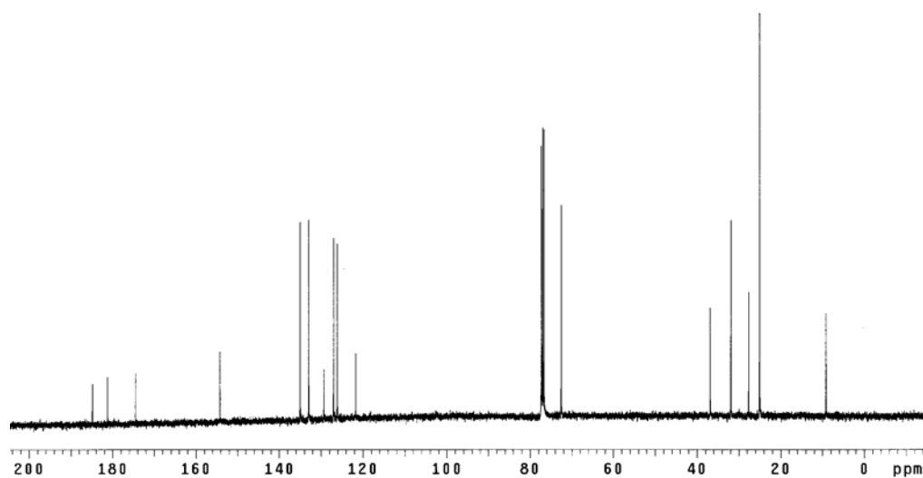
Appendix Figure 14 400 MHz 13 C NMR spectrum of 3-(1,4-dihydro-2-hydroxy-1,4-dioxonaphthalen-3-yl)-2,2-dimethylpropyl propionate ( 140 )
