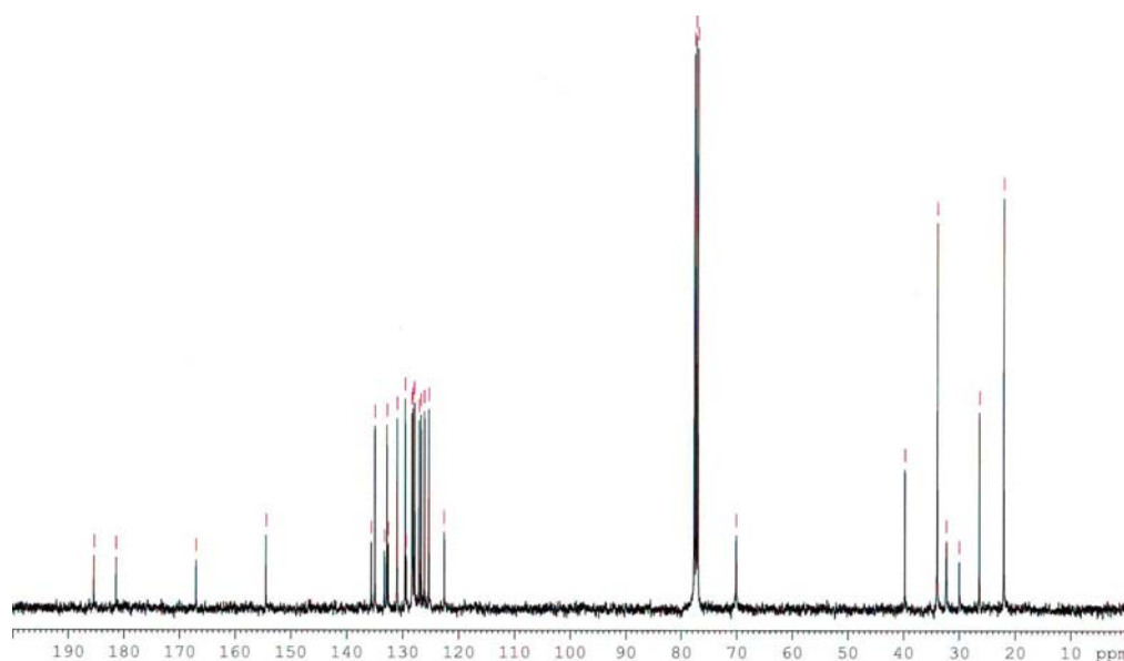
Appendix Figure 54 400 MHz ^{13}\text{C} NMR spectrum of (1-((1,4-dihydro-2-hydroxy-1,4-dioxonaphthalen-3-yl)methyl)cyclohexyl)methyl 2-methoxybenzoate ( 161 )
