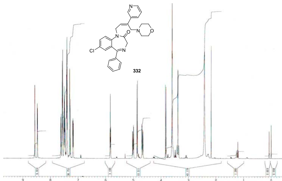
Appendix Figure 115 500 MHz ^{13}\text{C} NMR spectrum of 7-chloro-1-(4-morpholin-4-yl-3-pyridin-3-ylbut-2-enyl)-5-phenyl-1,3-dihydrobenzo[e][1,4]diazepin-2-one (332)
