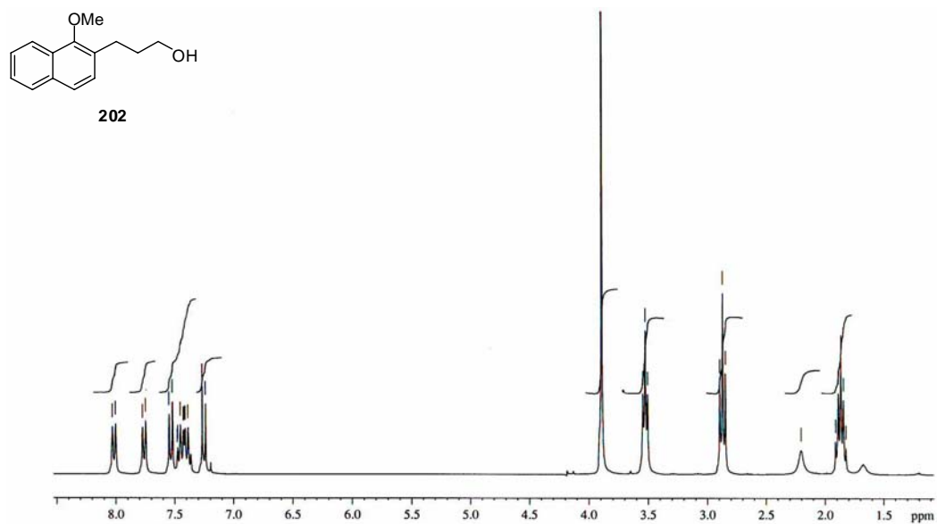
Appendix Figure 67 400 MHz 1 H NMR spectrum of 3-(1-methoxy-naphthalen-2-yl)-propan-1-ol ( 202 )
