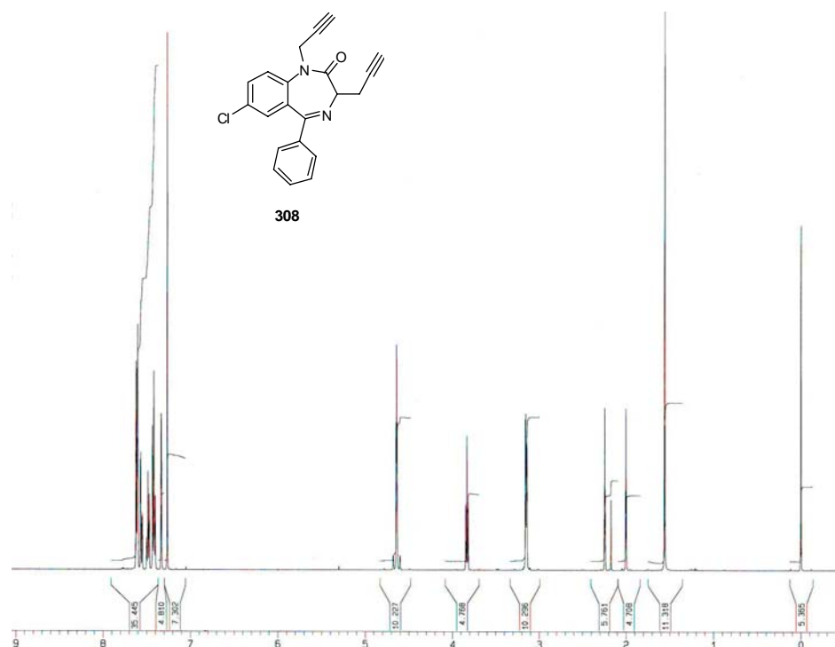
Appendix Figure 97 500 MHz ^{13}\text{C} NMR spectrum of 7-chloro-5-phenyl-1,3-diprop-2-ynyl-1,3-dihydro-benzo[e][1,4]diazepin-2-one ( 308 )
