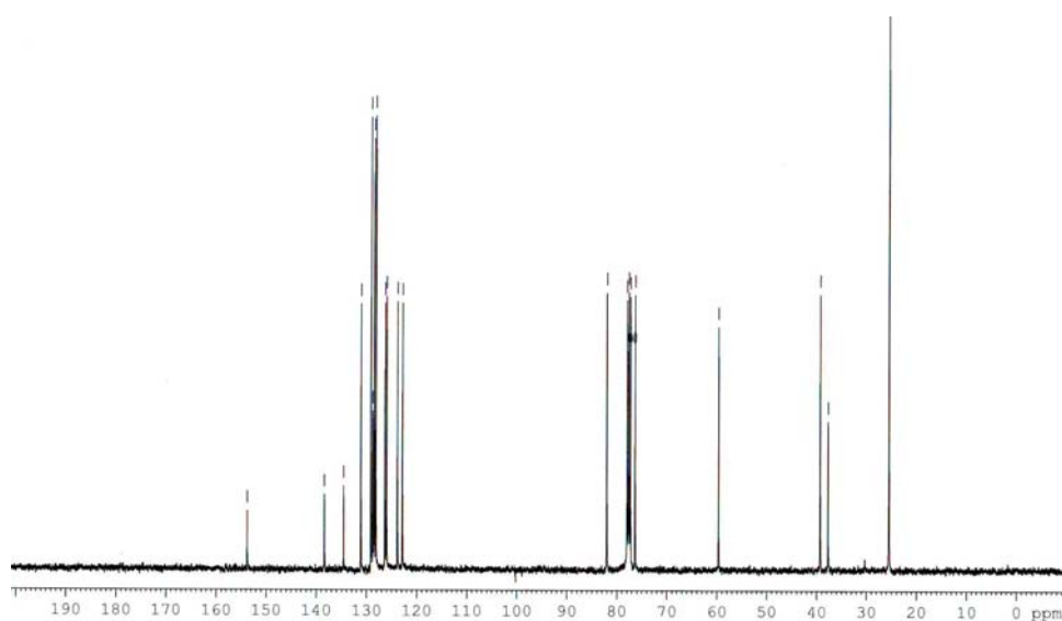
Appendix Figure 80 400 MHz 13 C NMR spectrum of 1-benzyloxy-2-(3-methoxy-2,2-dimethyl-propyl)-naphthalene ( 208 )
