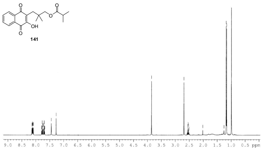
Appendix Figure 15 400 MHz 1 H NMR spectrum of 3-(1,4-dihydro-2-hydroxy-1,4-dioxonaphthalen-3-yl)-2,2-dimethylpropyl isobutyrate ( 141 )
