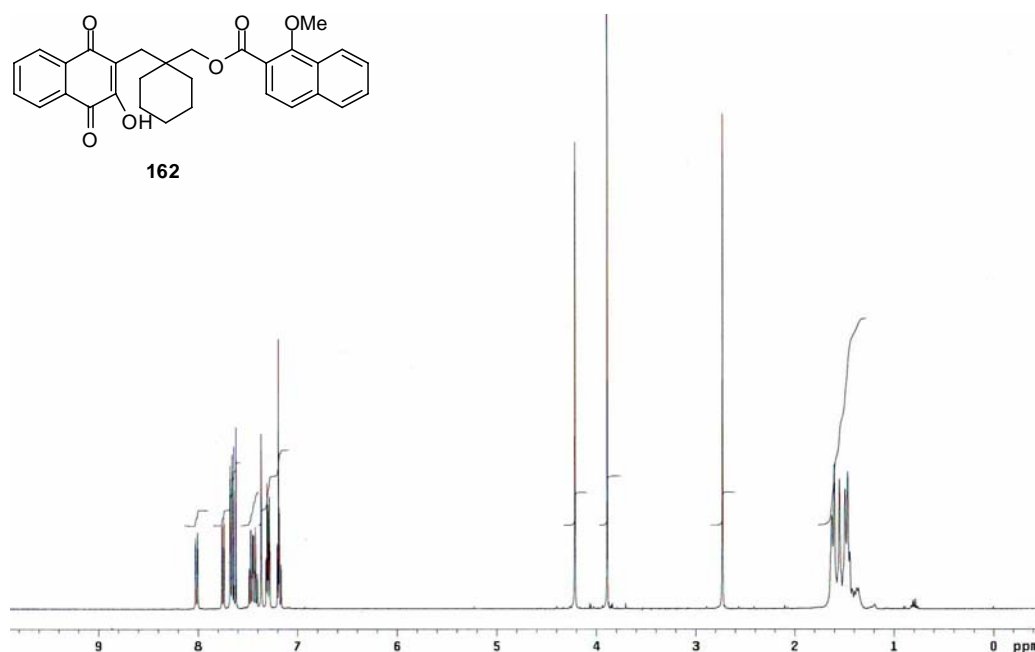
Appendix Figure 55 400 MHz ^1\text{H} NMR spectrum of (1-((1,4-dihydro-2-hydroxy-1,4-dioxonaphthalen-3-yl)methyl)cyclohexyl)methyl 1-methoxynaphthalene-2-carboxylate ( 162 )
