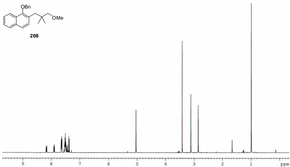
Appendix Figure 79 400 MHz 1 H NMR spectrum of 1-benzyloxy-2-(3-methoxy-2,2-dimethyl-propyl)-naphthalene ( 208 )
