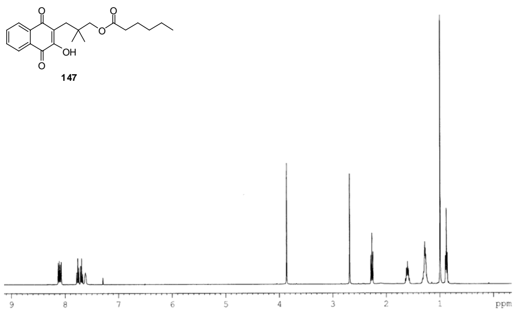
Appendix Figure 27 400 MHz 1 H NMR spectrum of 3-(1,4-dihydro-2-hydroxy-1,4-dioxonaphthalen-3-yl)-2,2-dimethylpropyl hexanoate ( 147 )
