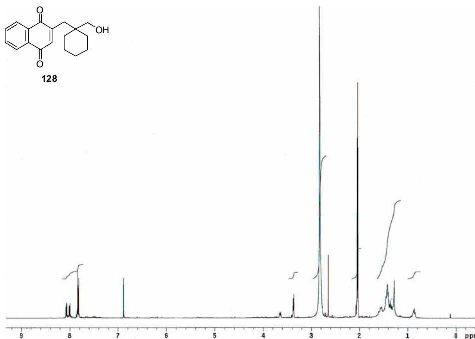
Appendix Figure 7 400 MHz 1 H NMR spectrum of 2-((1-(hydroxymethyl)cyclohexyl)methyl)naphthalene-1,4-dione ( 128 )
