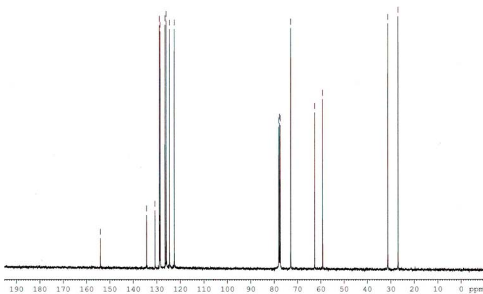
Appendix Figure 72 400 MHz 13 C NMR spectrum of 1-methoxy-2-(3-methoxypropyl)naphthalene ( 204 )
