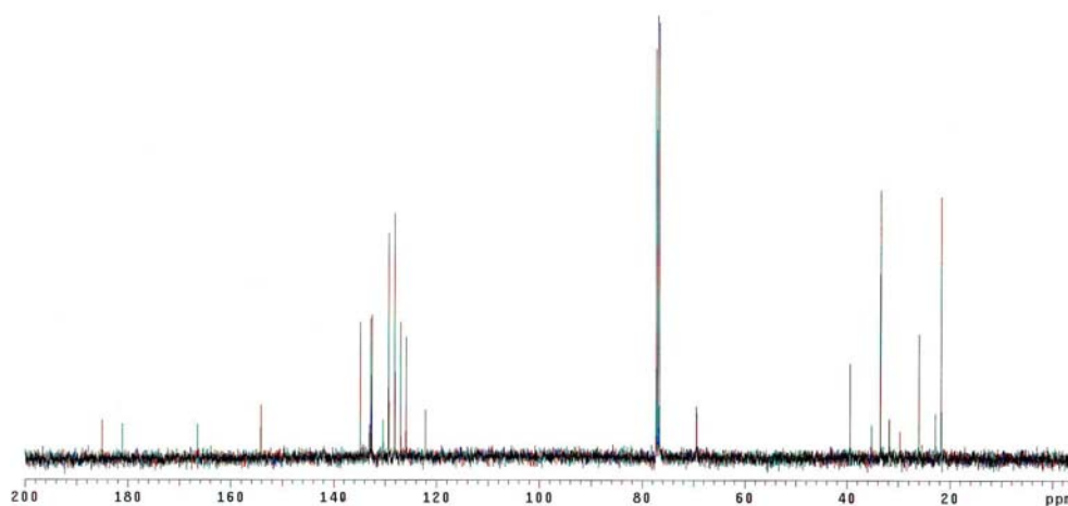
Appendix Figure 50 400 MHz ^{13}\text{C} NMR spectrum of (1-((1,4-dihydro-2-hydroxy-1,4-dioxonaphthalen-3-yl)methyl)cyclohexyl)methyl benzoate (159)
