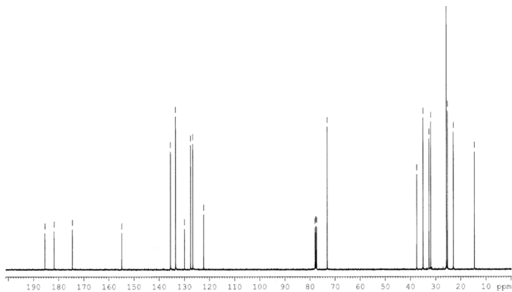
Appendix Figure 28 400 MHz 13 C NMR spectrum of 3-(1,4-dihydro-2-hydroxy-1,4-dioxonaphthalen-3-yl)-2,2-dimethylpropyl hexanoate ( 147 )
