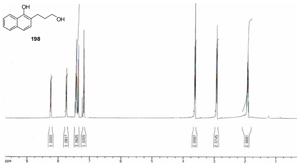
Appendix Figure 61 400 MHz ^1\text{H} NMR spectrum of 2-(3-hydroxy-propyl)-1-naphthalen-1-ol ( 198 )
