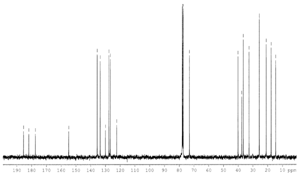
Appendix Figure 26 400 MHz 13 C NMR spectrum of 3-(1,4-dihydro-2-hydroxy-1,4-dioxonaphthalen-3-yl)-2,2-dimethylpropyl 2-methylpentanoate (146)
