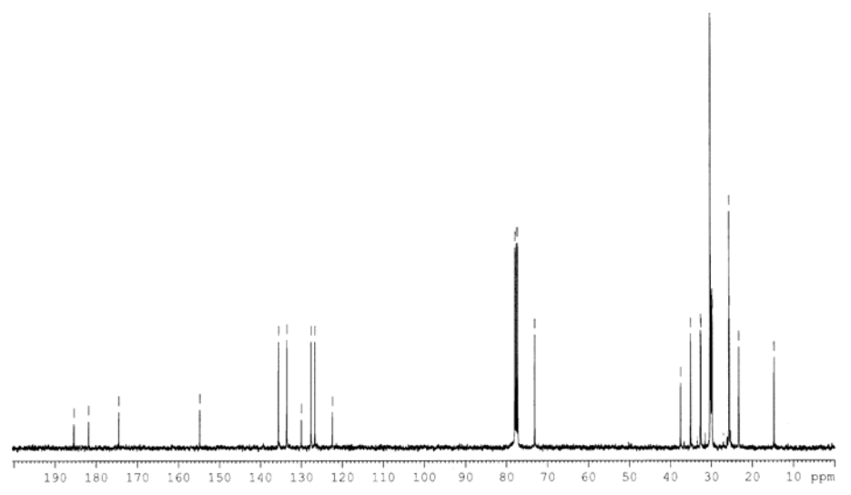
Appendix Figure 46 400 MHz 13 C NMR spectrum of 3-(1,4-dihydro-2-hydroxy-1,4-dioxonaphthalen-3-yl)-2,2-dimethylpropyl palmitate ( 156 )
