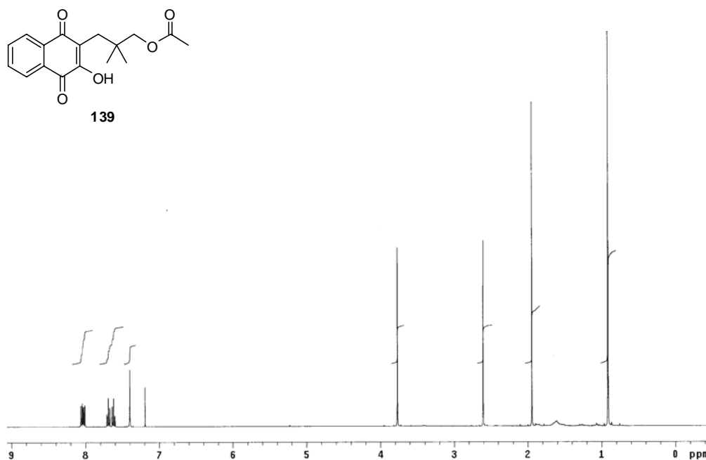
Appendix Figure 11 400 MHz 1 H NMR spectrum of 3-(1,4-dihydro-2-hydroxy-1,4-dioxonaphthalen-3-yl)-2,2-dimethylpropyl acetate ( 139 )
