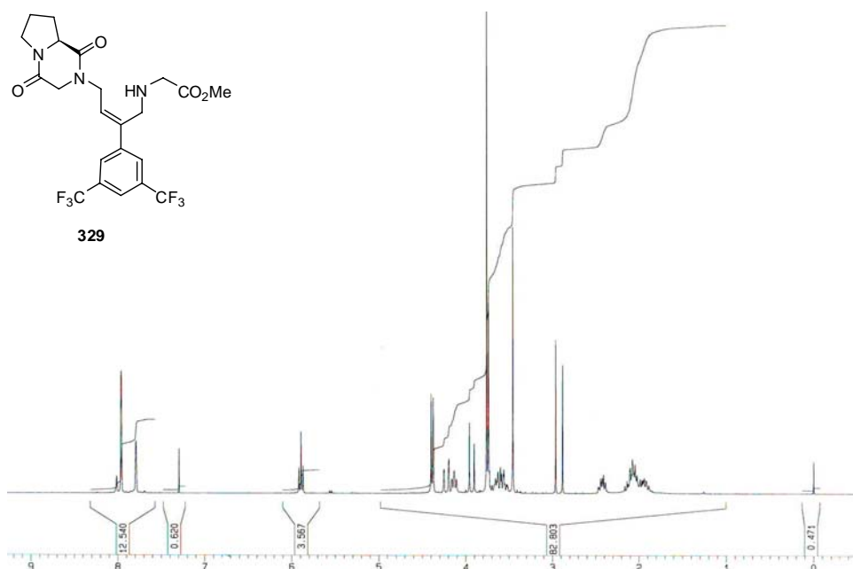
Appendix Figure 112 500 MHz ^{13}\text{C} NMR spectrum of [2-(3,5-bis-trifluoromethyl-phenyl)-4-(dioxo-hexahydro-pyrrolo[1,2-a]pyrazin-2-yl)-but-2-enylamino]-acetic acid methyl ester ( 329 )
