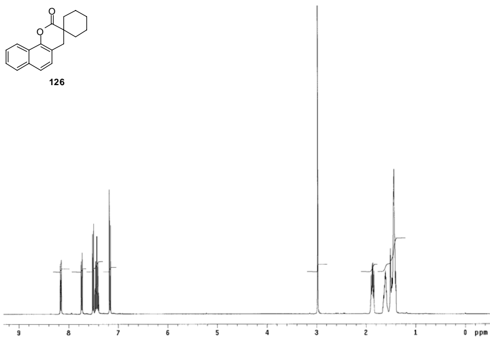
Appendix Figure 3 400 MHz 1 H NMR spectrum of 3,4-dihydro-2-spirocyclohexylbenzo[h]chromen-2-one ( 126 )
