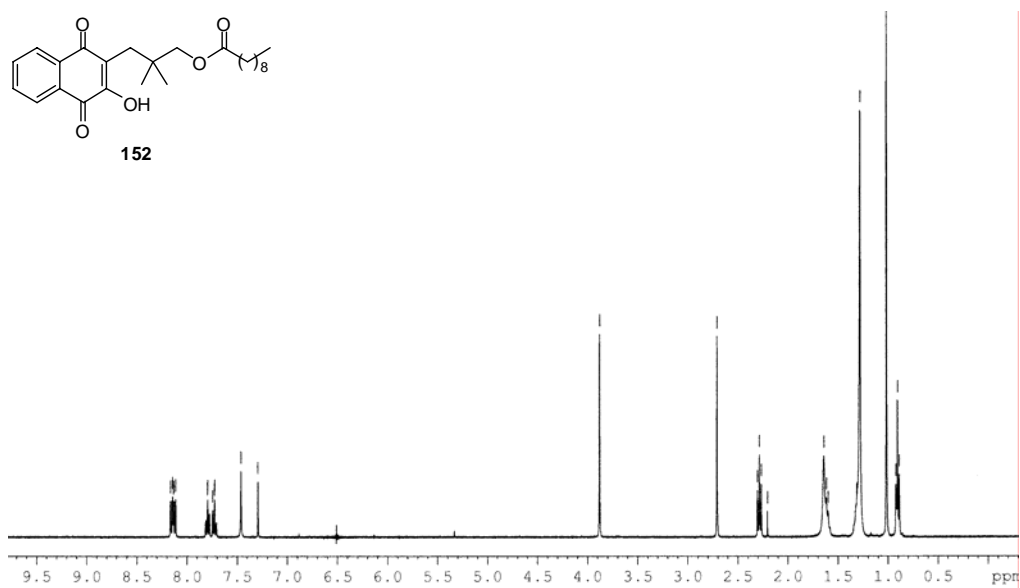
Appendix Figure 37 400 MHz 1 H NMR spectrum of 3-(1,4-dihydro-2-hydroxy-1,4-dioxonaphthalen-3-yl)-2,2-dimethylpropyl decanoate ( 152 )
