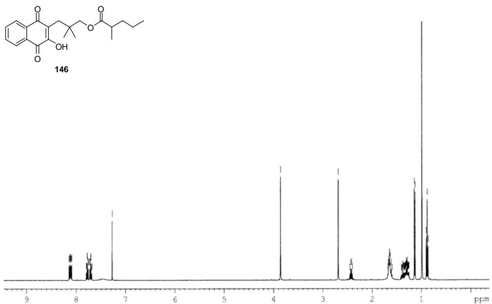
Appendix Figure 25 400 MHz 1 H NMR spectrum of 3-(1,4-dihydro-2-hydroxy-1,4-dioxonaphthalen-3-yl)-2,2-dimethylpropyl 2-methylpentanoate (146)
