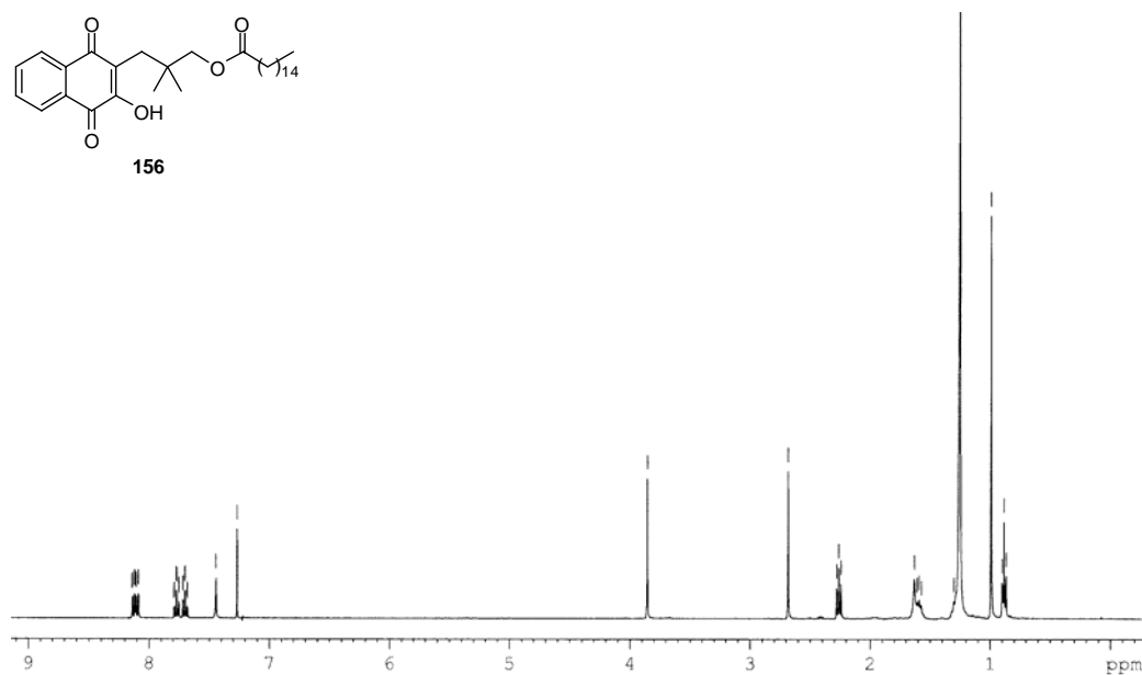
Appendix Figure 45 400 MHz 1 H NMR spectrum of 3-(1,4-dihydro-2-hydroxy-1,4-dioxonaphthalen-3-yl)-2,2-dimethylpropyl palmitate ( 156 )
