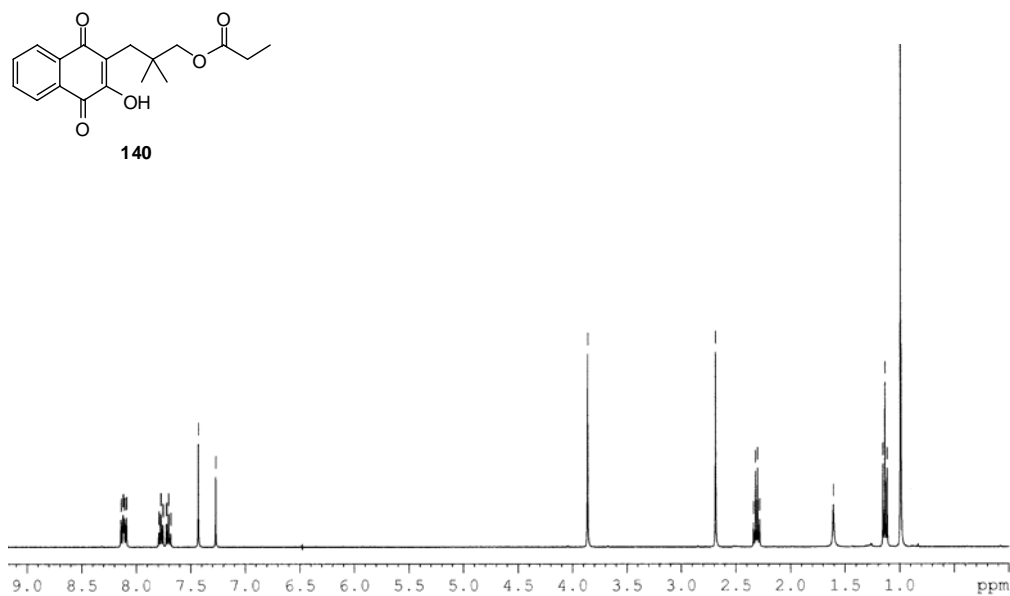
Appendix Figure 13 400 MHz 1 H NMR spectrum of 3-(1,4-dihydro-2-hydroxy-1,4-dioxonaphthalen-3-yl)-2,2-dimethylpropyl propionate ( 140 )
