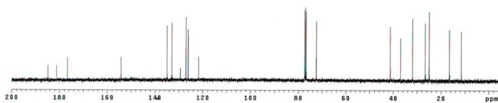
Appendix Figure 22 400 MHz 13 C NMR spectrum of (S)-3-(1,4-dihydro-2-hydroxy-1,4-dioxonaphthalen-3-yl)-2,2-dimethylpropyl 2-methylbutanoate ( 144 )
