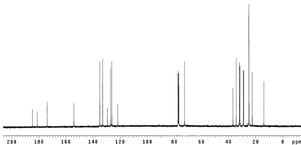
Appendix Figure 32 400 MHz 13 C NMR spectrum of 3-(1,4-dihydro-2-hydroxy-1,4-dioxonaphthalen-3-yl)-2,2-dimethylpropyloctanoate ( 149 )
