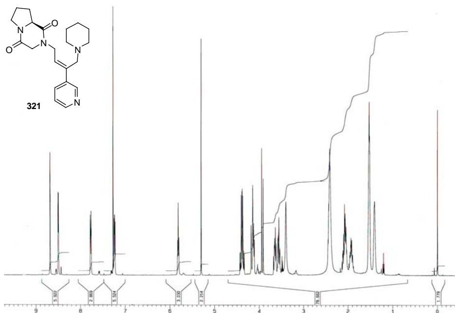
Appendix Figure 104 500 MHz ^{13}\text{C} NMR spectrum of 2-[(2Z)-4-piperidin-1-yl-3-pyridin-3-yl-but-2-en-1-yl]-hexahydro-pyrrolo[1,2-a]pyrazine-1,4-dione ( 321 )
