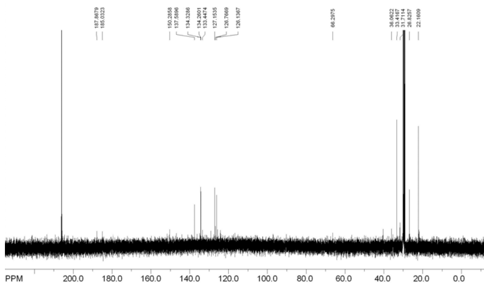
Appendix Figure 8 400 MHz 13 C NMR spectrum of 2-((1-(hydroxymethyl)cyclohexyl)methyl)naphthalene-1,4-dione ( 128 )
