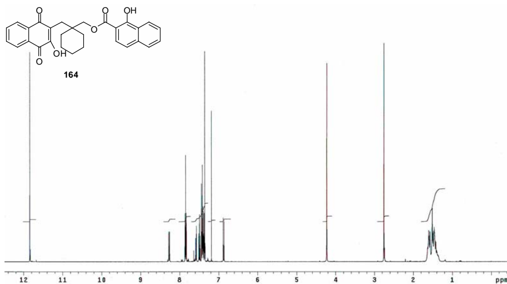
Appendix Figure 59 400 MHz ^1\text{H} NMR spectrum of (1-((1,4-dihydro-2-hydroxy-1,4-dioxonaphthalen-3-yl)methyl)cyclohexyl)methyl 1-hydroxynaphthalene-2-carboxylate ( 164 )
