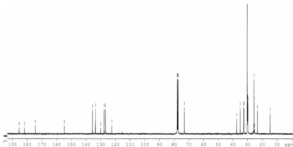
Appendix Figure 48 400 MHz 13 C NMR spectrum of 3-(1,4-dihydro-2-hydroxy-1,4-dioxonaphthalen-3-yl)-2,2-dimethylpropyl stearate ( 157 )
