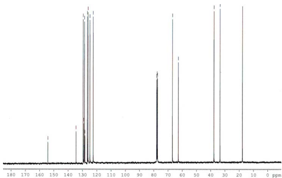
Appendix Figure 70 400 MHz 13 C NMR spectrum of 3-(1-methoxy-naphthalen-2-yl)-2-methyl-propan-1-ol ( 203 )
