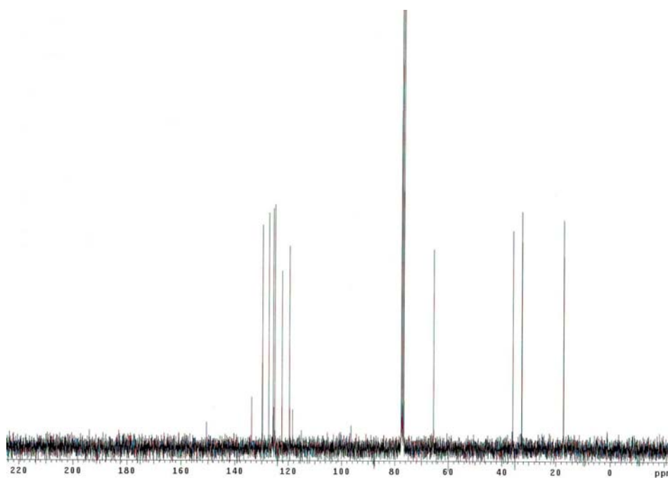
Appendix Figure 64 400 MHz ^{13}\text{C} NMR spectrum of 2-(3-hydroxy-2-methylpropyl)-naphthalen-1-ol ( 199 )
