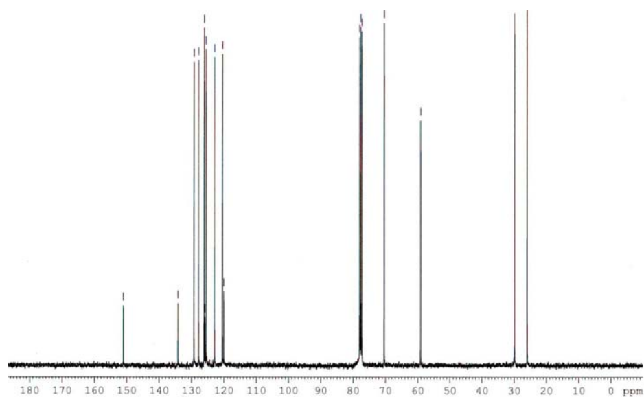
Appendix Figure 74 400 MHz ^{13}\text{C} NMR spectrum of 2-(3-methoxy-propyl)-naphthalen-1-ol ( 205 )
