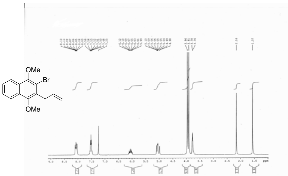
Appendix Figure 5 300 MHz 1 H NMR spectrum of 2-allyl-3-bromo-1,4-dimethoxynaphthalene (116)
