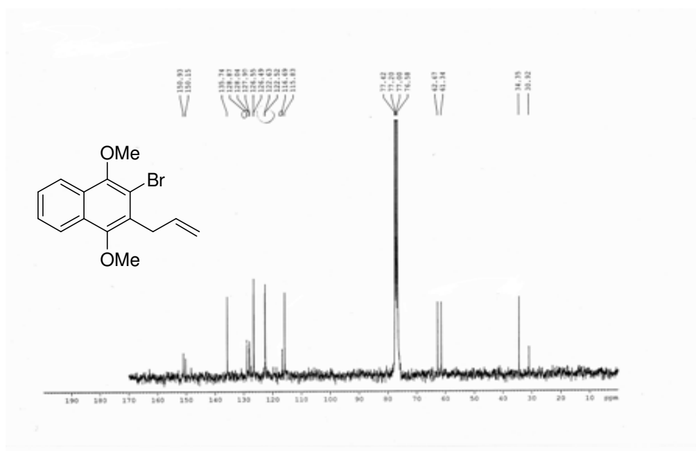
Appendix Figure 6 100 MHz 13 C NMR spectrum of 2-allyl-3-bromo-1,4-dimethoxynaphthalene (116)
