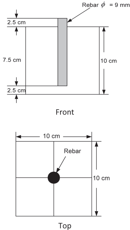
Figure 4 Conceptual sketch of specimens
