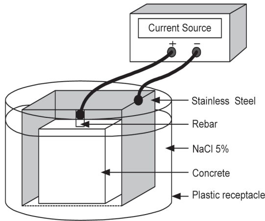
Figure 5 Conceptual sketch of electric current was used to accelerate the corrosion
