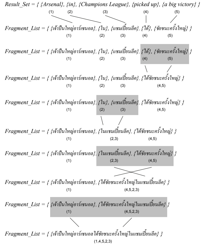
Fig. 2. n -gram generation component by example
