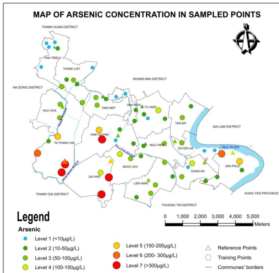
Figure 1 Arsenic concentration in sampled points
