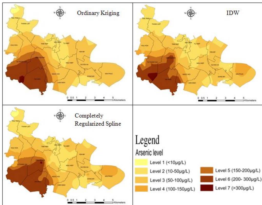
Figure 2 Surfaces of arsenic concentration produced by the three interpolators
