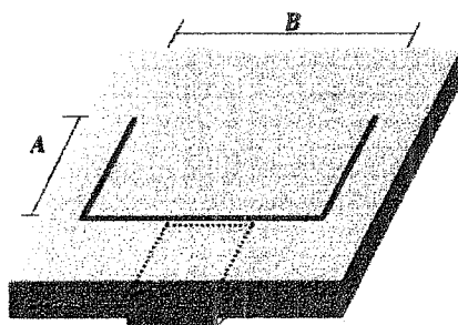
Figure 2. U-shape slot antenna structure.
