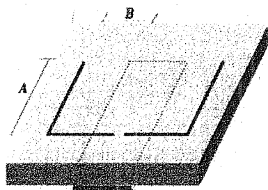
Figure 1. Double-L shape slot antenna structure.
