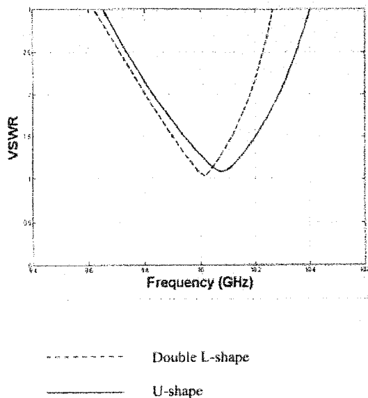
Figure 4. VSWR of two shape antennas.
