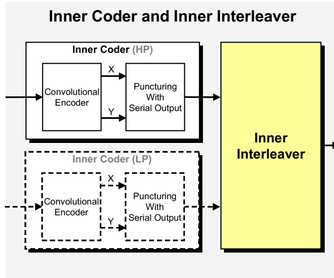
Figure 6: Inner coding and interleaving
