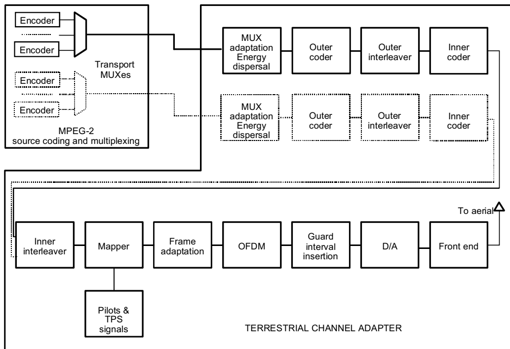
Figure 1: Functional block diagram of the System
