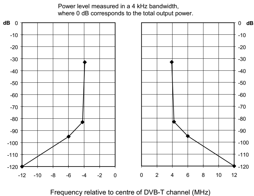
Figure 14: Spectrum mask for critical cases
