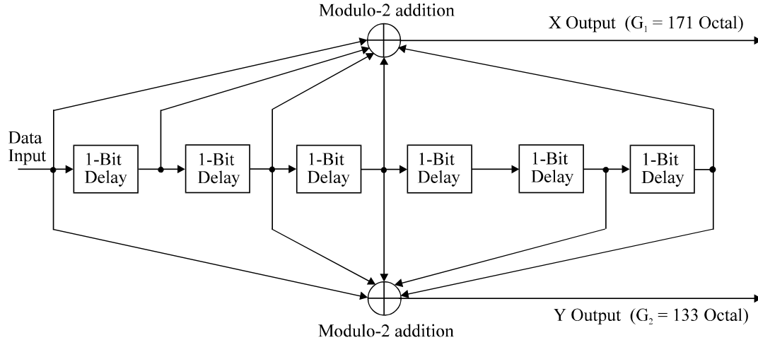
Figure 5: The mother convolutional code of rate 1/2
