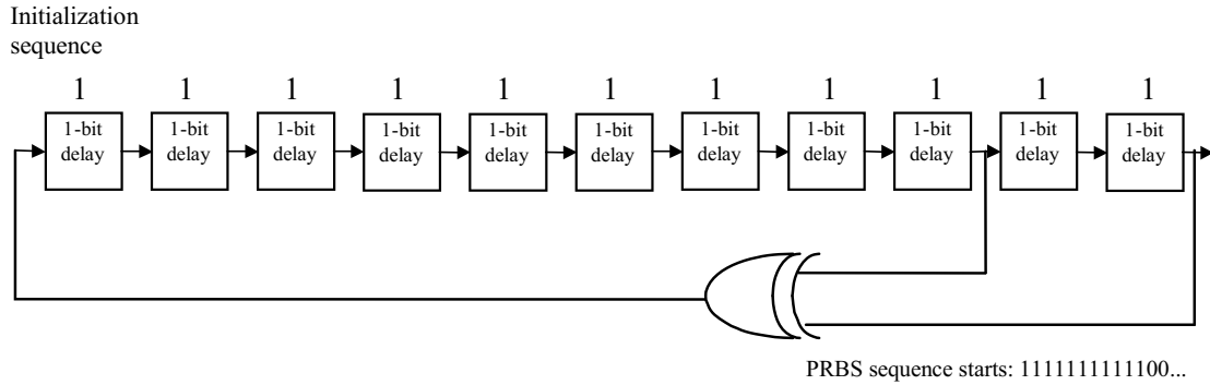
Figure 10: Generation of PRBS sequence
