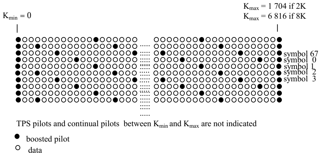
Figure 11: Frame structure
