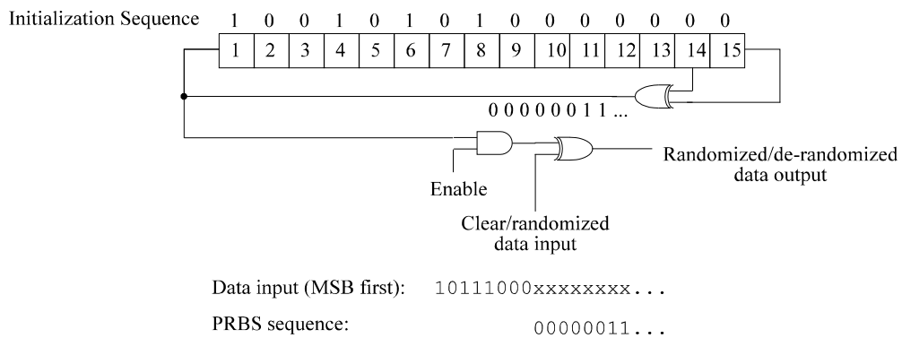
Figure 2: Scrambler/descrambler schematic diagram
