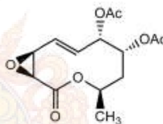
Lactone [7]
