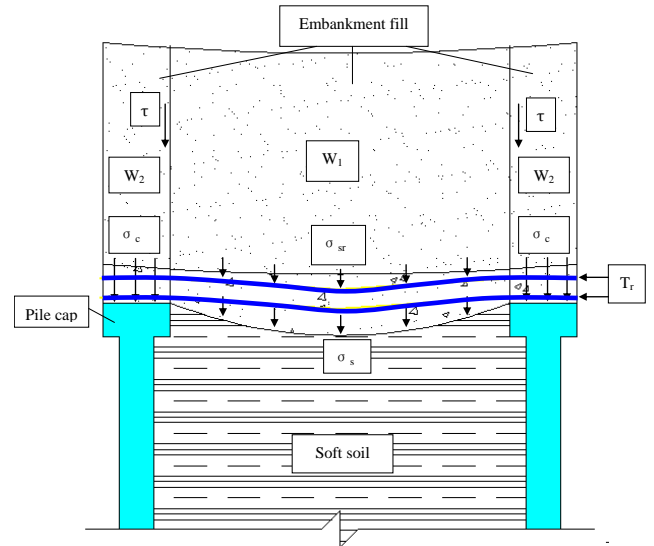
Figure 21 Stress and force generated in GRPS embankment
