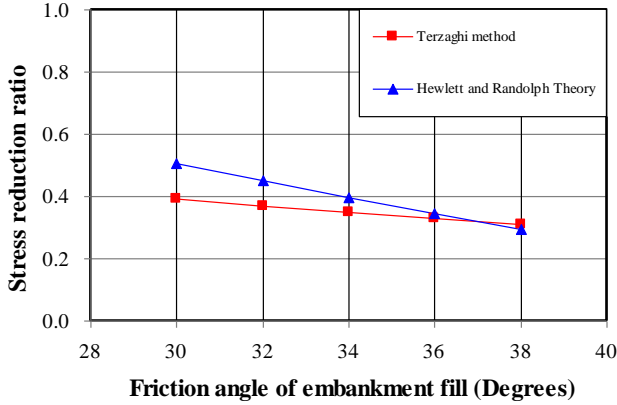
Figure 28 Influence of friction angle of embankment on S_{3D}
