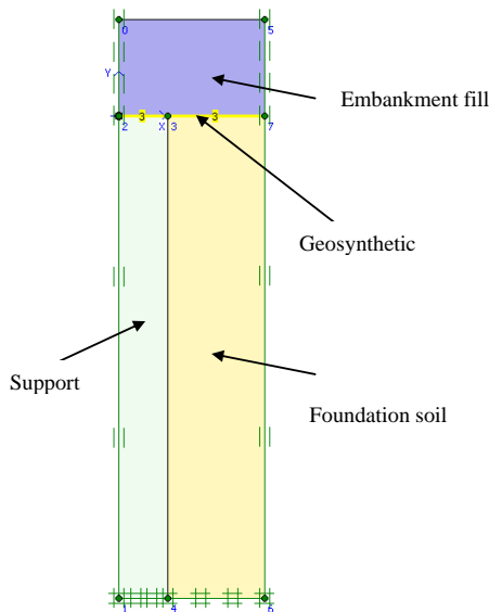
Figure 30 Geometry of axis-symmetric model
