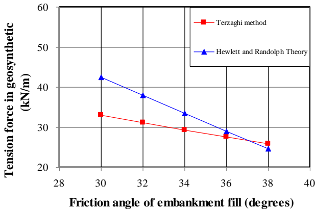
Figure 29 Influence of friction angle of embankment on tensile force in geogrids
