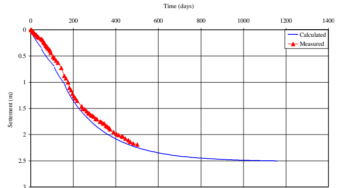
Figure 9 Calculated and measured settlement
