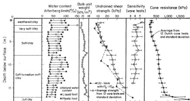
Figure 4(b) RTN Dockyard site in Bangkok Plain (Balasubramaniam et al. , 1980)
