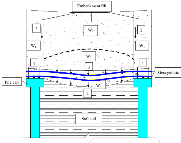
Figure 20 Load transfer mechanisms of GRPS embankment
