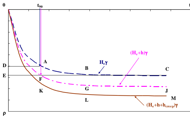
Figure 8(b) Settlement-time graph corresponds to embankment load H_c\gamma
