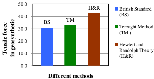
Figure 24 Comparison of tensile force in geogrid calculated from four analytical methods
