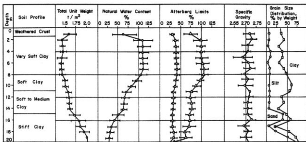
Figure 4(a) Bangkok Swarnabhum Airport site (Moh et al. , 1969, Moh and Woo, 1987)
