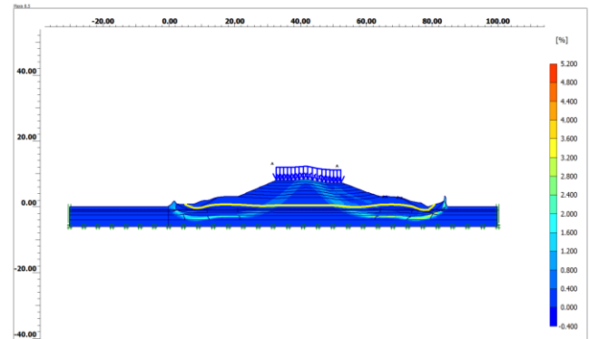
Figure 19 Wedge type of failure from Plaxis
