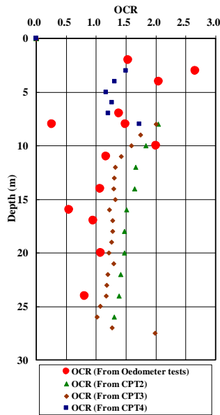
Figure 13 OCR with depth
