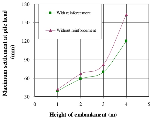
Figure 32 Influence of embankment height on maximum settlement
