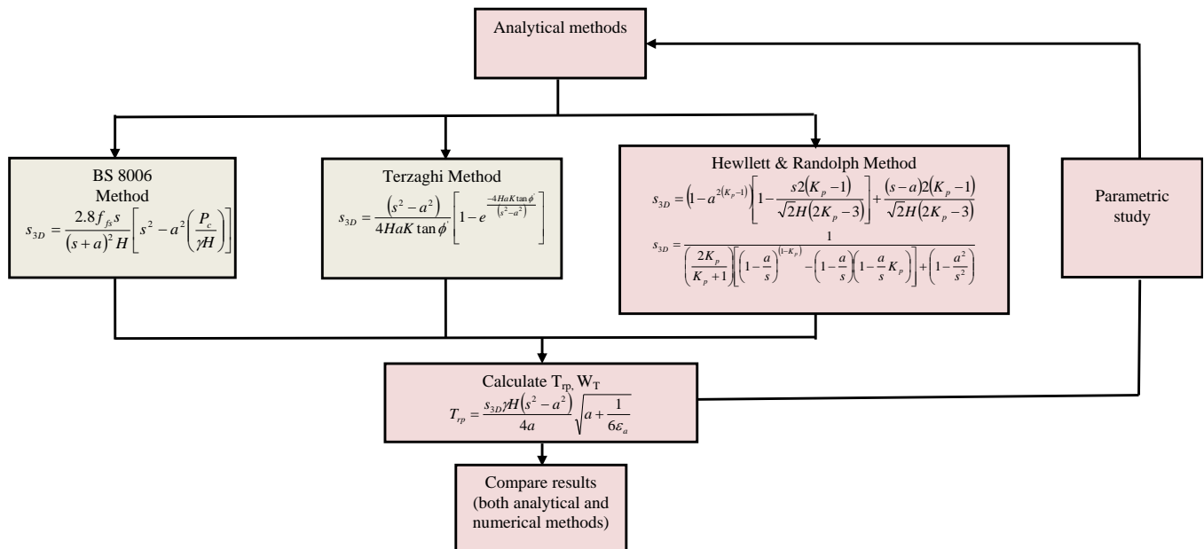
Fig. 22 Procedure adopted in the use of analytical methods in GPRS embankments
