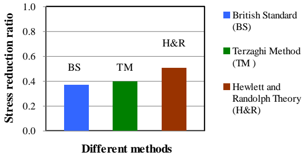
Figure 23 Comparison of stress reduction ratio calculated from four analytical methods
