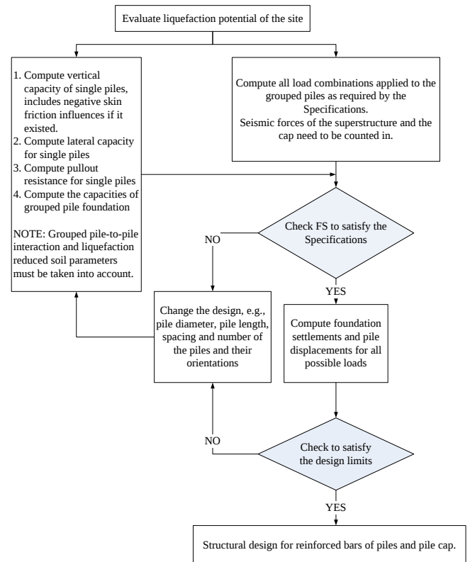
Fig. 2 Common pile design procedures undertaken in Taiwan
