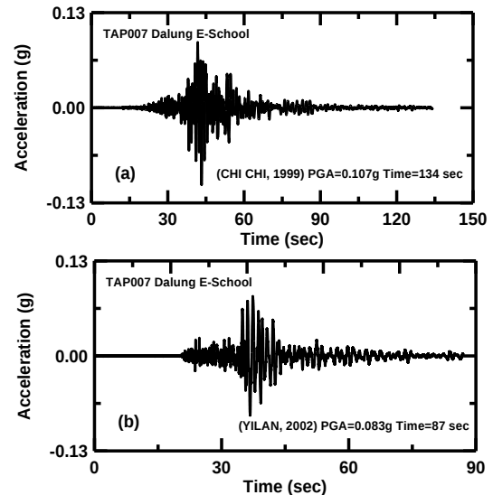
Fig. 6 Accelergram records of (a) Chi-Chi and (b) Yi-Lang EQs
