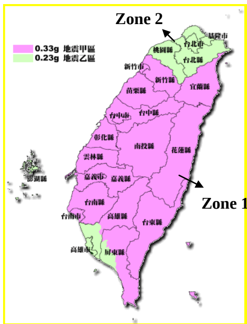
Fig. 4 Seismic zones suggested in old seismic design code in Taiwan
