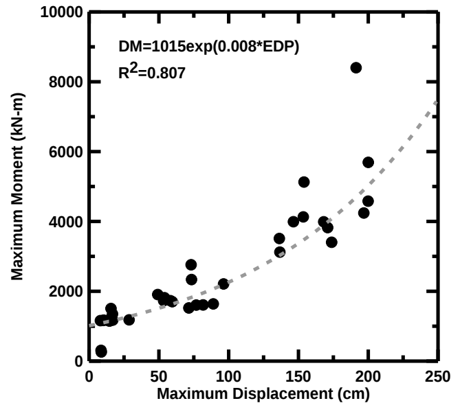
Fig.12 Maximum bending moments vs. maximum pile displacements for single pile located in Taipei Basin
