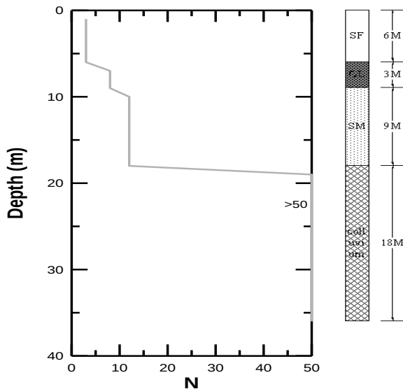
Fig. 9 Ground profile used at the site of pile foundation
