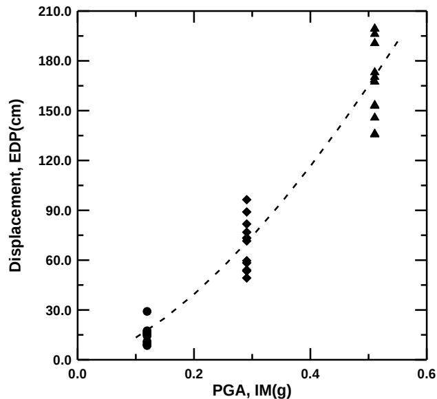
Fig. 10 Demand curve of EDP medians based on target PGAs
