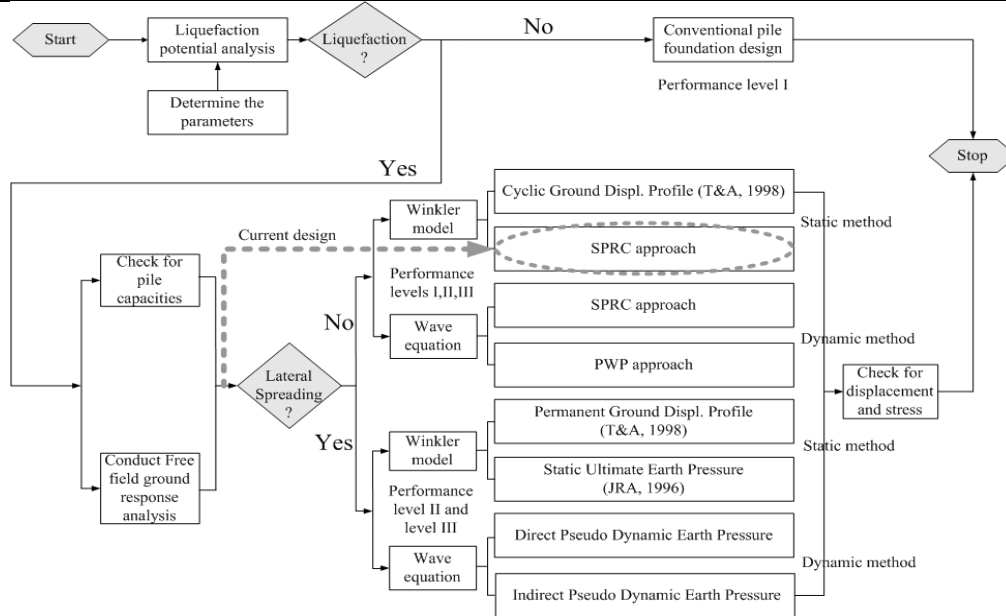
Fig. 3 Seismic performance-based design procedures and methods suggested for pile design in Taiwan
