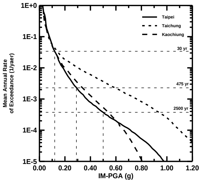
Fig. 5 Hazard curves of Taipei, Taichung and Kaoshiung (based on total mean curves by Cheng, 2002)
