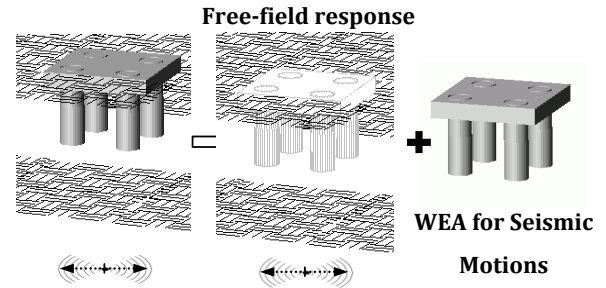
Fig. 1 Uncoupled procedures used in EQWEAP
