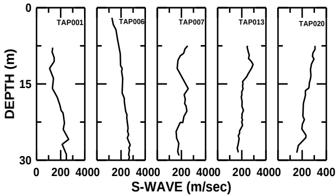
Fig. 8 Velocity profiles at the seismic stations at Taipei City
