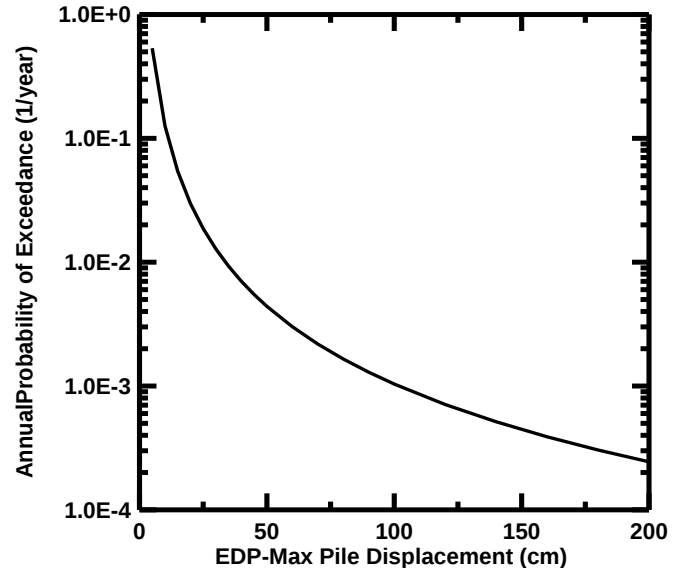
Fig. 11 Mean annual rate of exceedance for various EDPs
