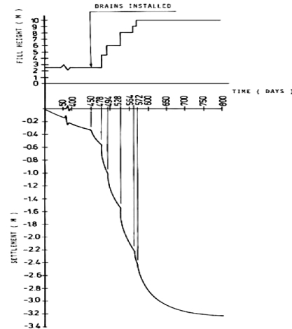
Fig. 6 Time-settlement curve at the coal storage yard, Port Kelang Power Station (Risseuw et al. , 1986)
