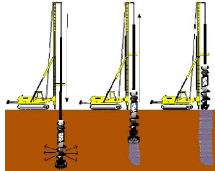
Fig. 30 Installation of CMC by displacement
