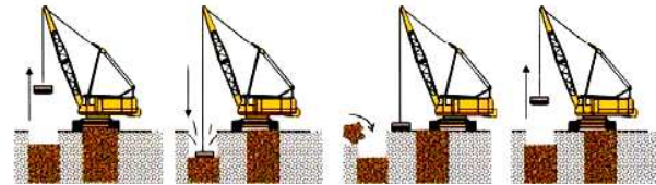
Fig. 27 Columns formed by dynamic replacement (DR) process
