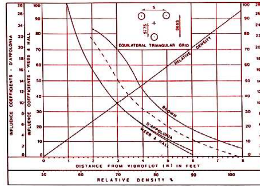
Fig. 21 Area pattern design chart (Glover, 1982)
