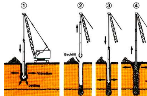
Fig. 24 Installation of stone columns by top feed wet method
