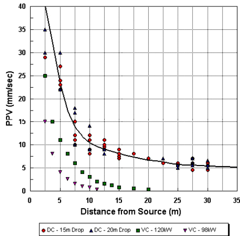
Fig. 22 PPV for dynamic compaction (DC) using 15-ton pounder and vibro compaction (VC)
