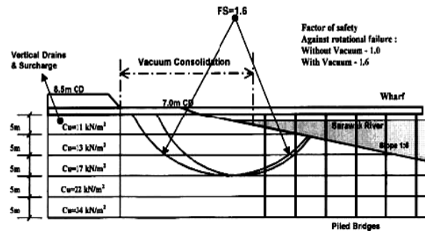
Fig. 11 Simplified cross-section of ground improvement scheme for the New Kuching Deepwater Port
