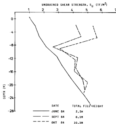
Fig. 5 Shear strength increase after consolidation at the coal storage yard, Port Kelang Power Station (Risseuw et al. , 1986)
