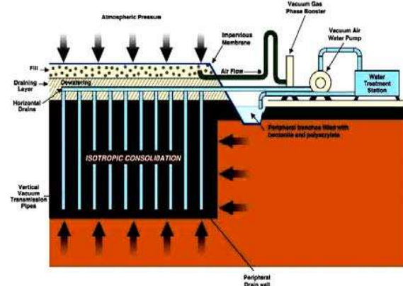
Fig. 9 Schematic layout of a vacuum consolidation system
