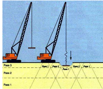
Fig. 13 Various phases of dynamic compaction process
