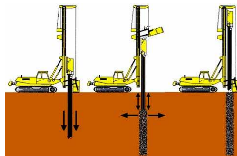
Fig. 25 Installation of stone columns by bottom feed dry method
