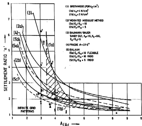
Fig. 33 Settlement ratio curves with reinforcement granular columns (Greenwood & Kirsch, 1983)
