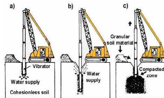
Fig. 20 Vibro compaction process
