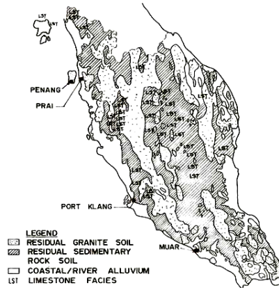
Fig. 3 Geological map of Peninsular Malaysia (Ting, 1985)
