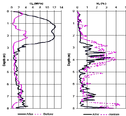
Fig. 18 CPT results before and after SVC at Bidor - Kampar
