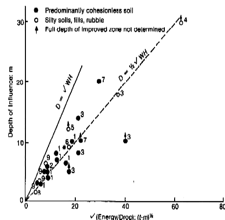
Fig. 14 Compaction energy against depth of influence / treatment depth (Green & Kirsch, 1983)
