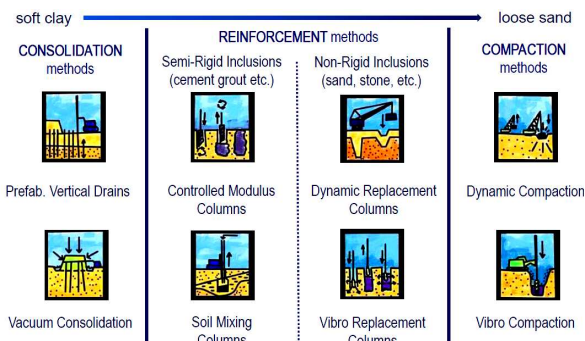
Fig. 2 Common ground improvement techniques
