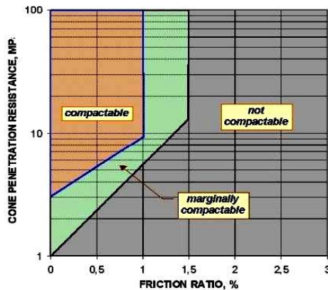
Fig. 23 Soil compactability according to CPT results (Massarch & Heppel, 1991)
