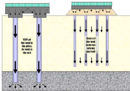
Fig. 29 Concept of CMC columns compared with RC piles
