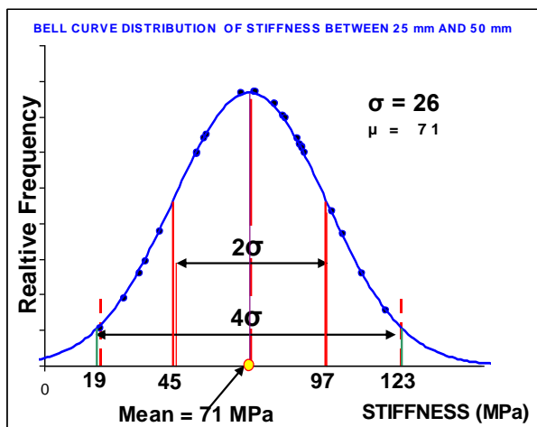
Figure 23 Relative frequency of stiffness response for loads causing movements of 25 mm and 50 mm
