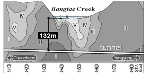
Figure 19 Tunnel beneath the creek
