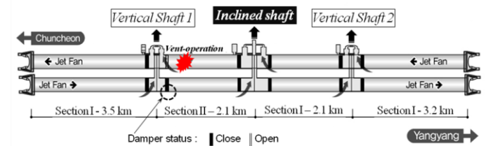
Figure 29 Ventilation plan for the fire in the tunnel
