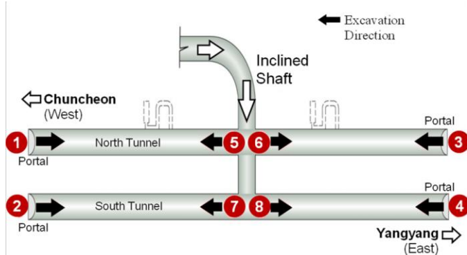
Figure 34 Excavation directions (8 points)
