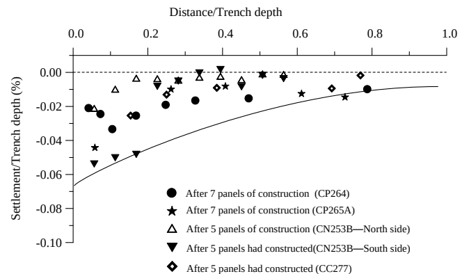
Figure 14 Normalized ground settlement due to the construction of multiple panels
