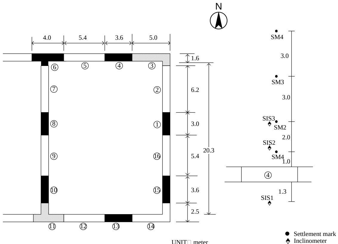
Figure 9 Paneling of the CN255 contract and its monitoring items
