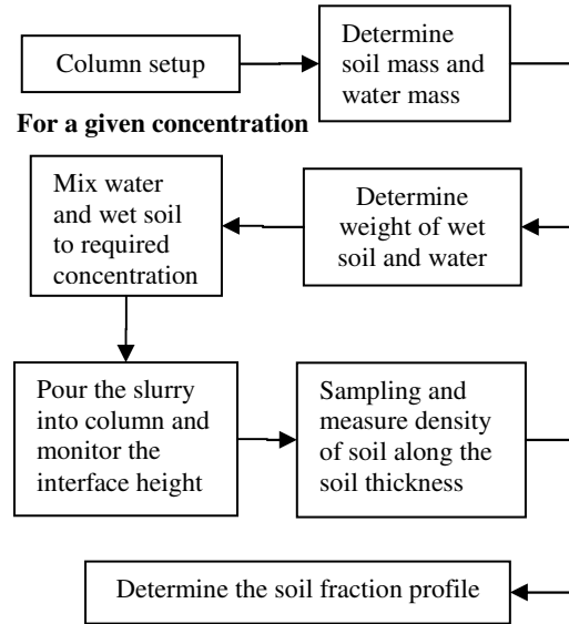
Figure 2 Flow chart of the experiment procedure
