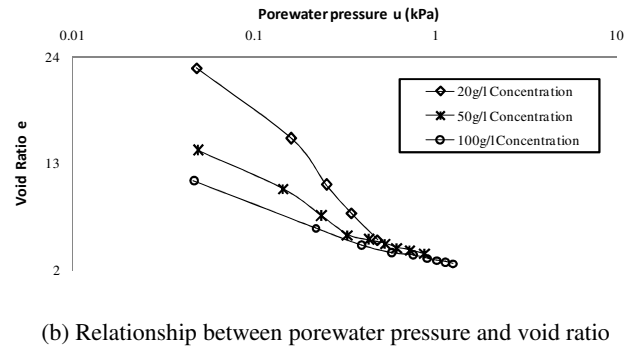
Figure 5 Consolidation of sample 19
