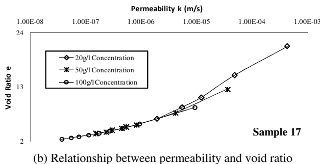
Figure 4 Consolidation behavior of sample 17
