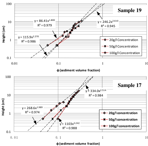
Figure 6 Relationship between sediment height and volume fraction
