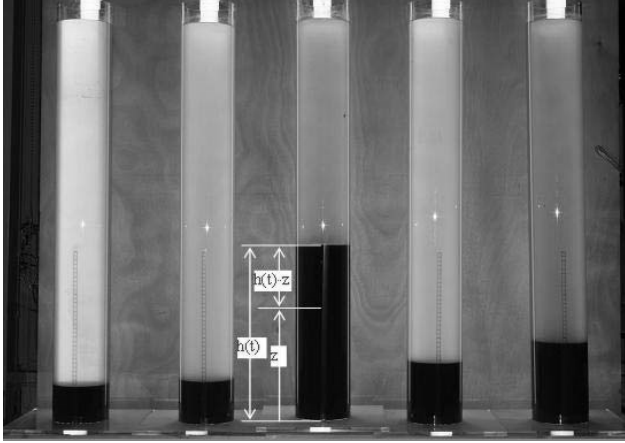
Figure 1. Column setup for settling column tests. (advised by Delft Hydraulics, 2007)
