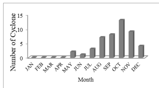
Figure 3 Monthly tropical data over 20 years
