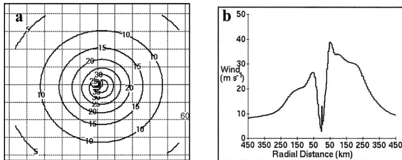
Figure 1 Relationship between wind speed and the radius of maximum wind speed
