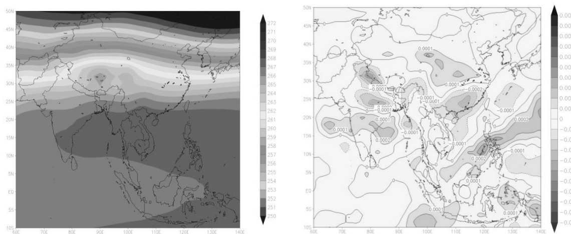
Figure 9 ECMWF temperature data at 200 hPa (1989) and temperature differences at 200 hPa (1989)
