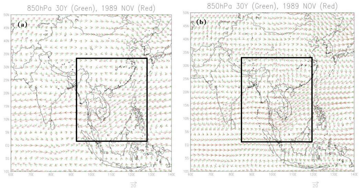
Figure 7 Average 30-year winds (green) using wind data from November 1989 (red). (a) ECMWF data (b) NCEP data
