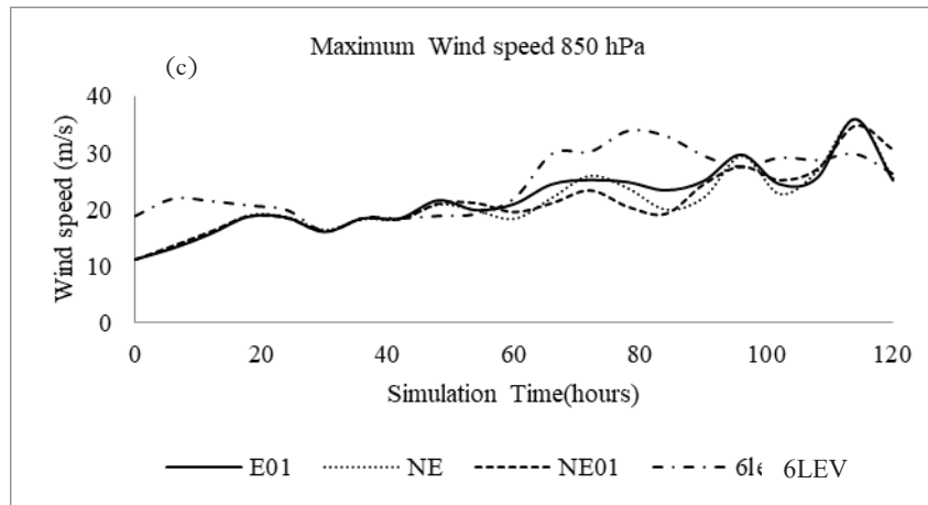
Figure 11 Maximum wind speed at 10 m, 925 hPa, 850 hPa and 200 hPa
