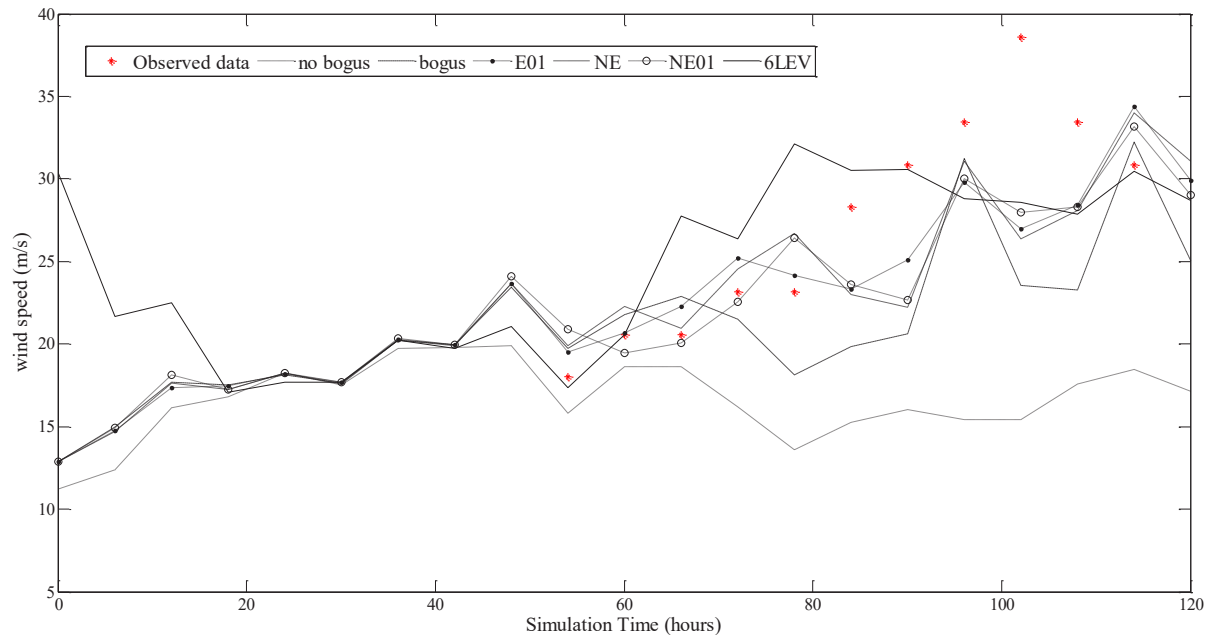
Figure 13 Maximum wind speed at 925 hPa
