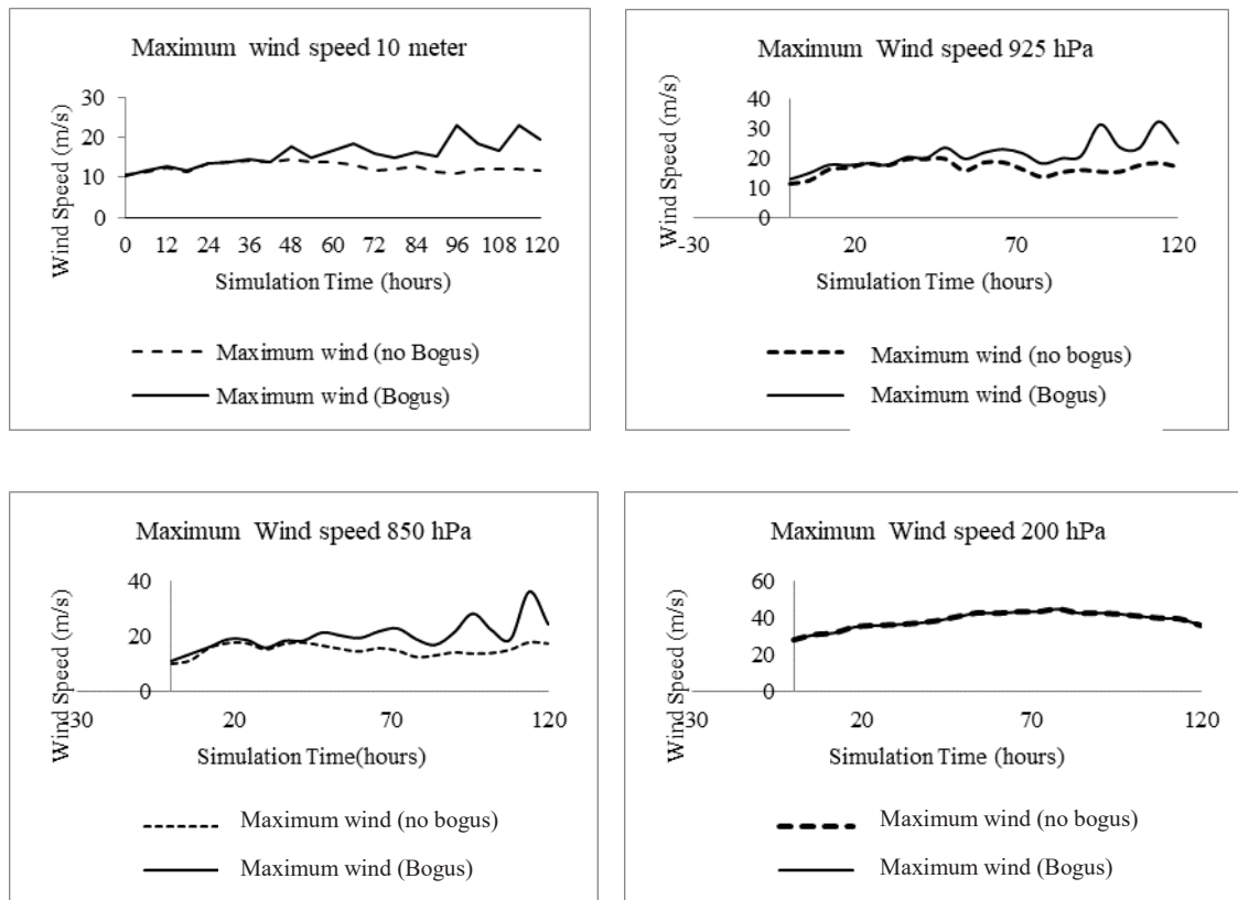
Figure 10 Maximum wind speeds at 10 m, 925 hPa, 850 hPa, and 200 hPa
