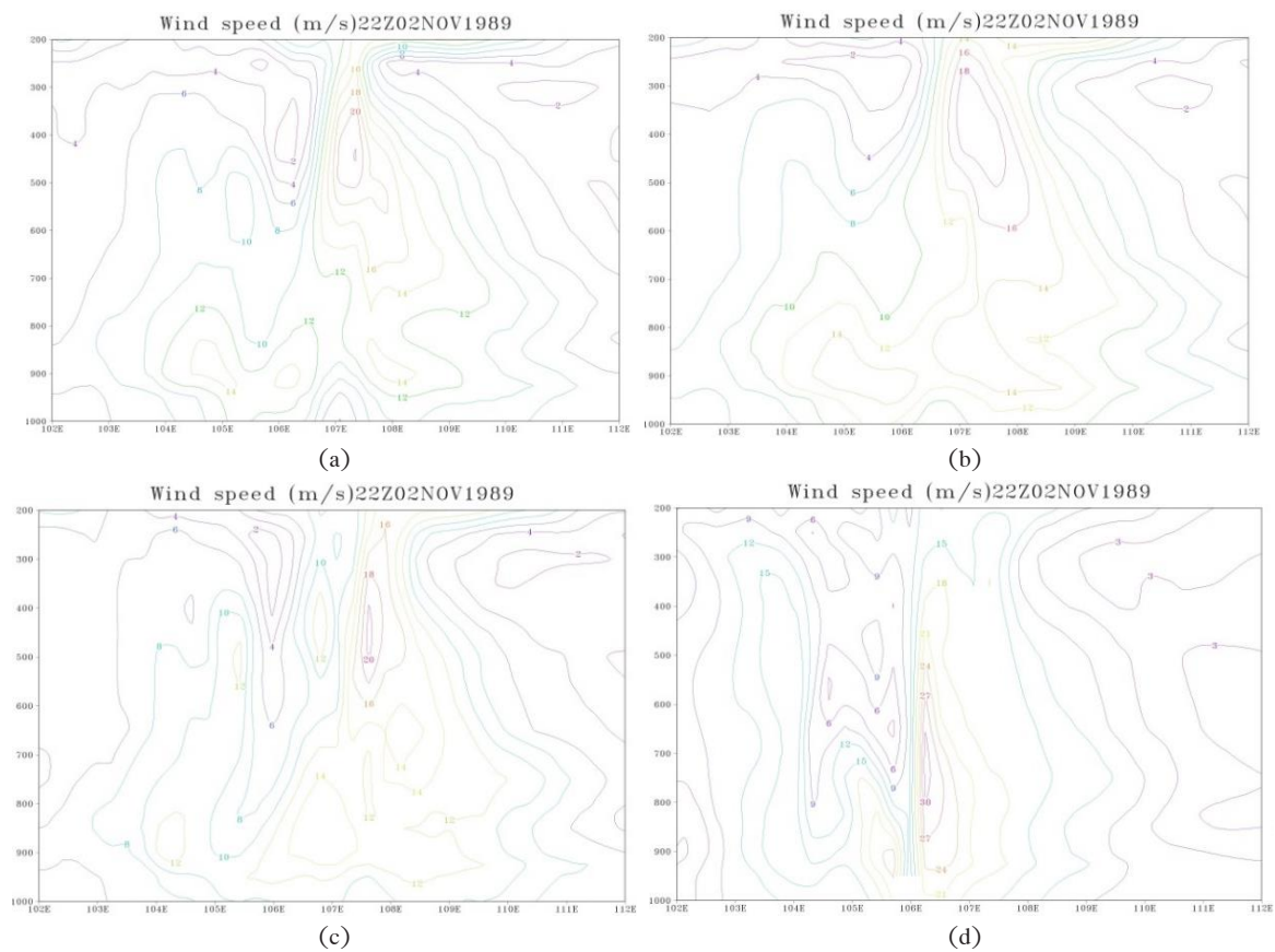
Figure 12 Cross section of the tropical cyclone on November 2, 1989. (a) Control, (b) Rankin vortex initialization, (c) northeast u-v wind adjustment at 3 levels, and (d) northeast u-v wind adjustment at 6 levels
