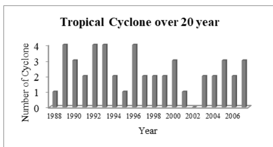
Figure 2 Tropical data from 1988–2007
