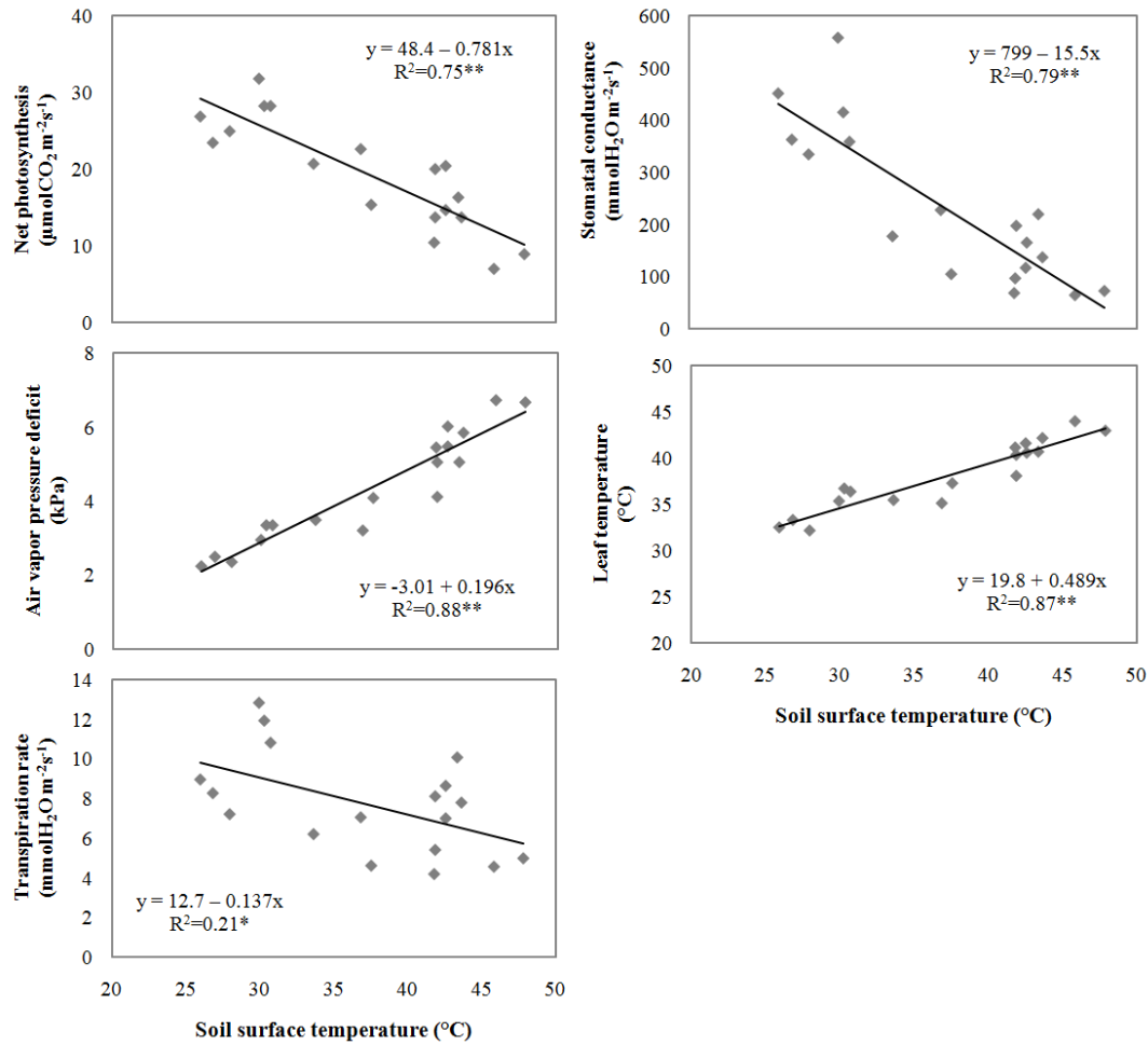
Figure 3 Correlation between surface soil temperature and cassava physiological parameters.
