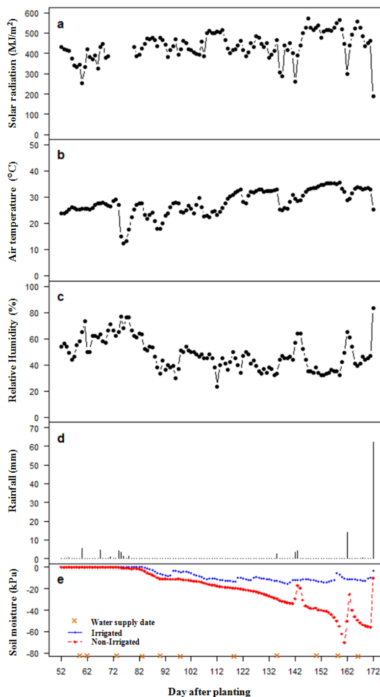
Figure 1 Daily data of the weather and soil moisture in the field experiment during field measurement.
