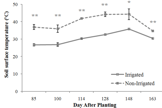
Figure 2 The average of surface soil temperature in the cassava irrigated and non-irrigated plot.
