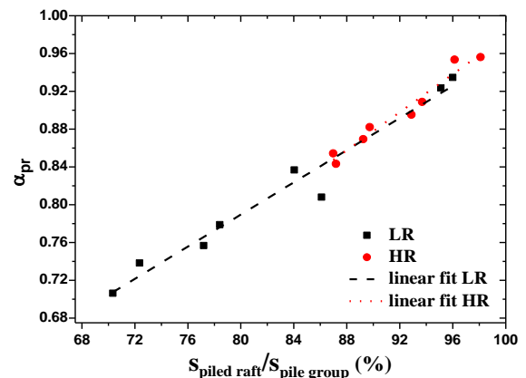
Figure 12 Relation of load sharing ratio by piles in PRF and the ratio of settlements of PRF and PG low rise and high rise buildings
