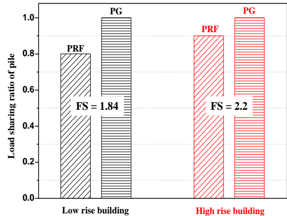
Figure 11 Load shared by piles of PRF and PG between Low rise and High rise buildings with 2 basements
