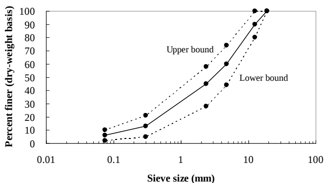
Figure 1. Gradation of aggregate
