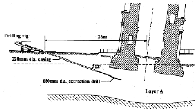
Figure 11 Soil extraction from beneath the north side of the Pisa Tower
