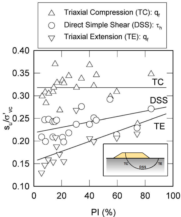
Figure 5 Undrained Strength Ratio used on Embankments over Soft Ground
