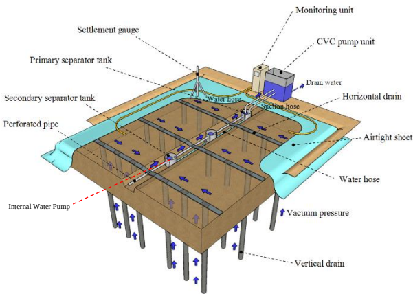
Figure 7 Vacuum System with Double Pumps
