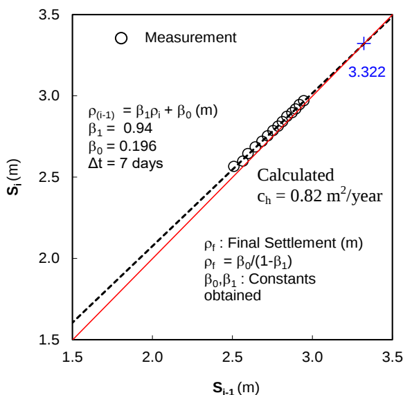
Figure 11 Asaoka Method on Section A
