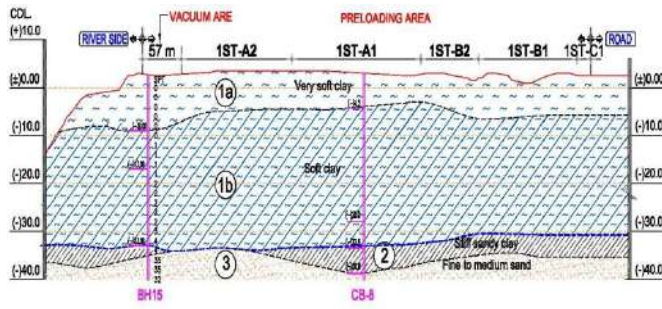
Figure 2 Soil profile at the site
