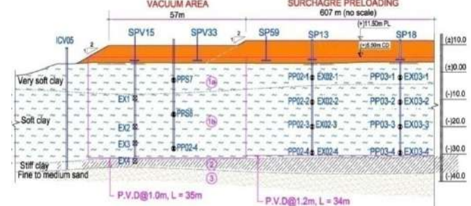
Figure 9 Typical cross sections
