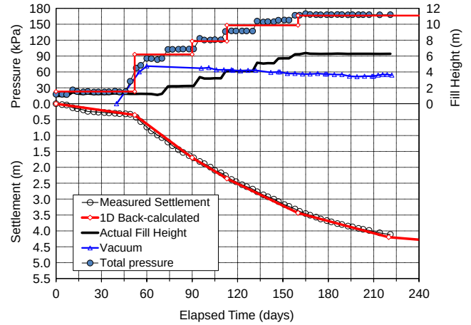
Figure 23 Back calculation of settlement at SP-V15 of VCA
