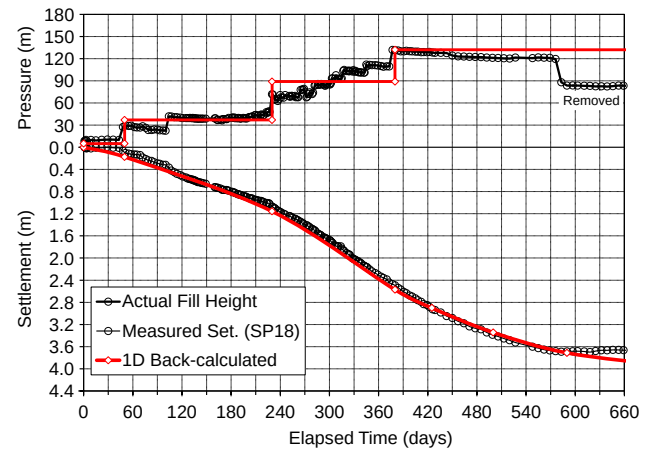
Figure 24 Back calculation of settlement at SP-18 of SPA
