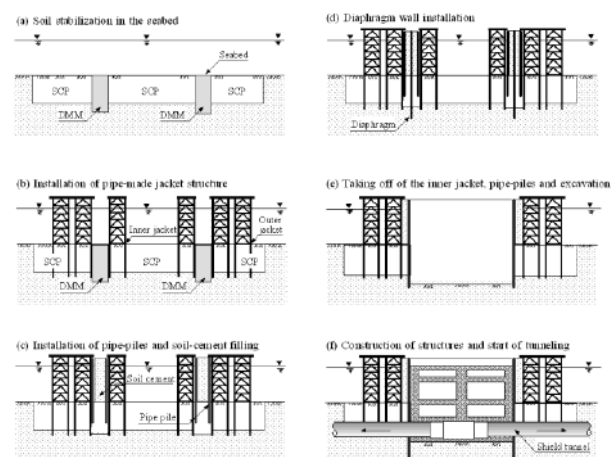
Figure 46 Construction process of the man-made Island
