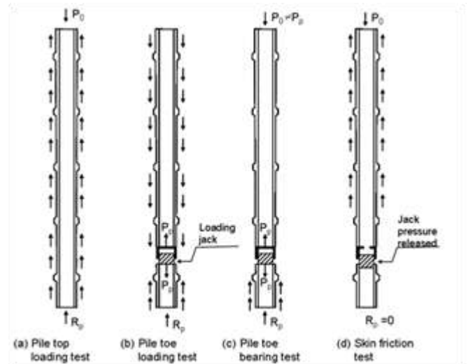
Figure 9 Four types of pile loading test
