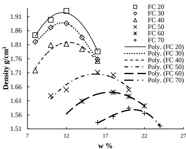
Figure 3 Compaction curves
