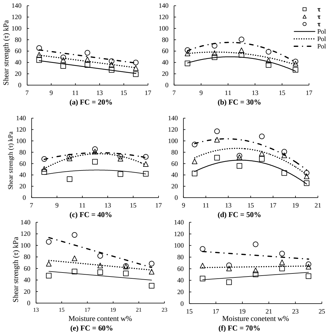
Figure 7 Shear strength versus moisture content at different fine content
