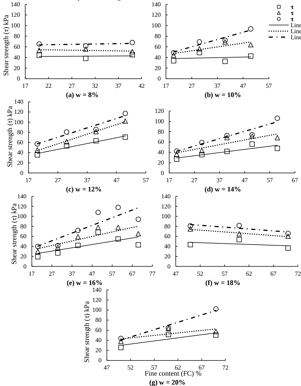
Figure 10 Shear strength versus fine content at different moisture content
