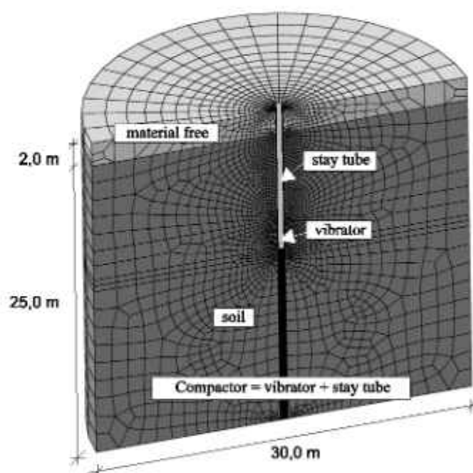
Figure 2 Vertical cut through the three dimensional CEL-model to simulate the deep vibration compaction method.
