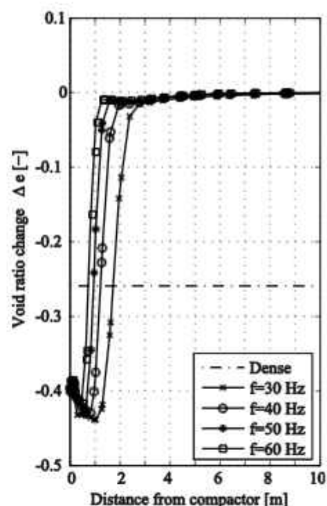
Figure 4 Void ratio change along a horizontal path halfway down the depth vibrator for a displacement controlled simulation with a horizontal displacement of the tip of the vibrator of 12 mm with varying vibration frequency according to Henke et al. (2012)
