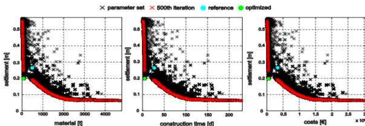
Figure 8 Results of multicriterial optimization with multiple objectives: reduction of settlements, material demand, costs and construction time; possible parameter sets are marked with crosses, the last generation is highlighted in red; the chosen reference design is marked with a blue circle and one optimized design is marked with a green circle
