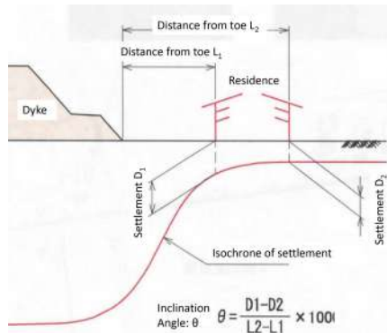
Figure 22 Inclination angle
