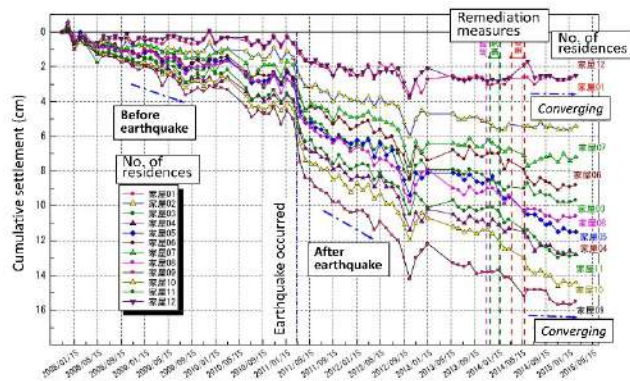
Figure 6 Settlement vs. time curves for residences.
