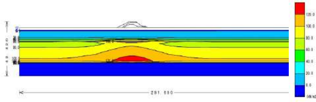
Figure 14 Distribution of EPWP generated by the earthquake
