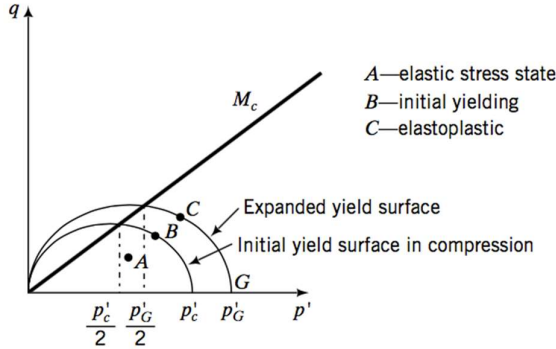
Figure 1 Yield surface of Cam-Clay model (Budhu, 2010)
