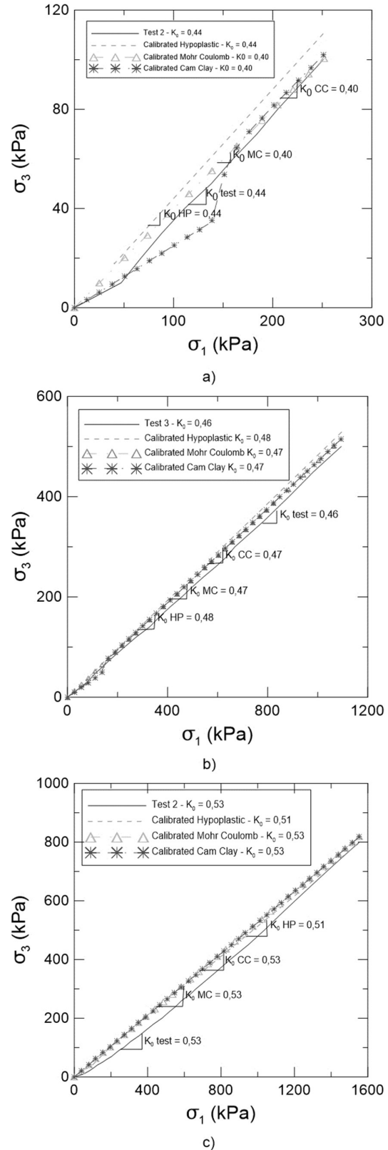
Figure 13 Numerical simulation results. a) Sample 1, b) Sample 2., c) Sample 3
