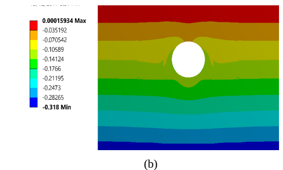
Figure 4 Vertical Stresses in Soils for (a) B/D = 1.5 and (b) B/D = 5
