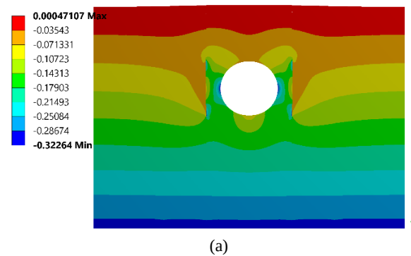
Figure 3 Horizontal Soil Reaction in the Horizontal Plane for B/D = 1.5, 3, 5
