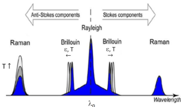
Figure 3 Typical spontaneous scattering spectrum from an optical glass fiber
