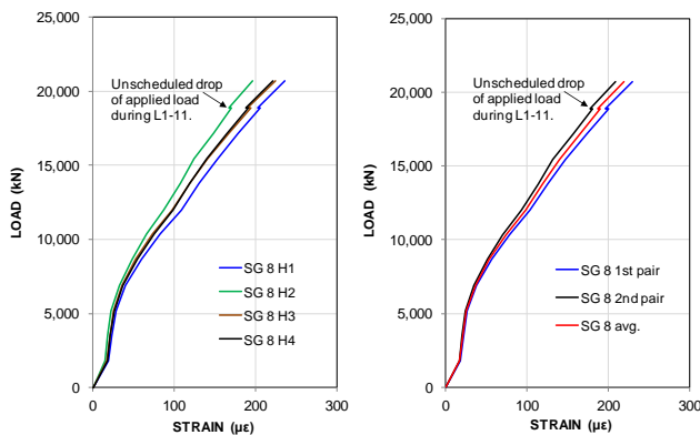
Figure 25 Case 4 Strain records at SGL8: single-gage, pair averages, and average of all gages
