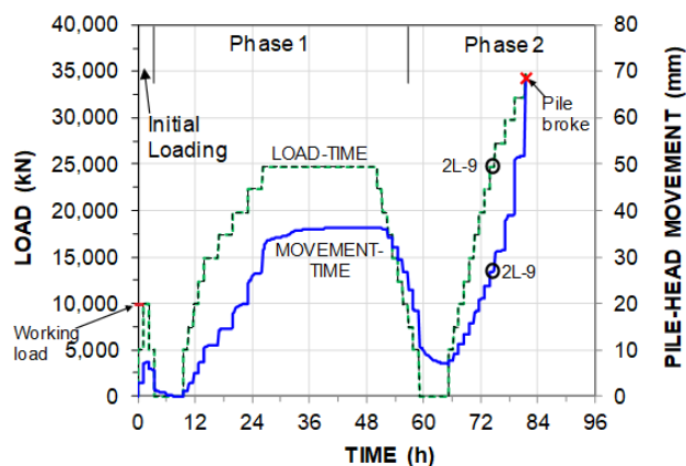
Figure 6 Case 3. Load-time
