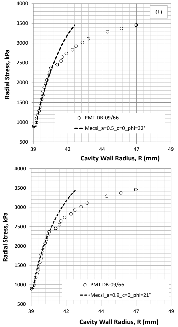
Figure 6 No Unique c - \phi values obtained by Mecsi Formulas
