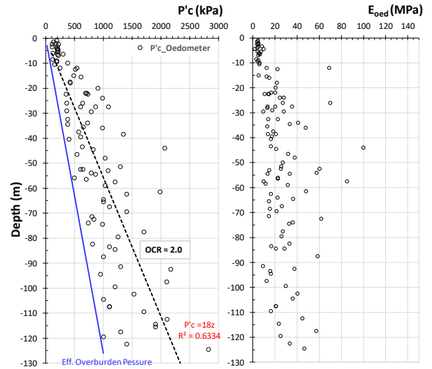
Figure 12 Pre-Consolidation Pressures and Oedometer Modulus
