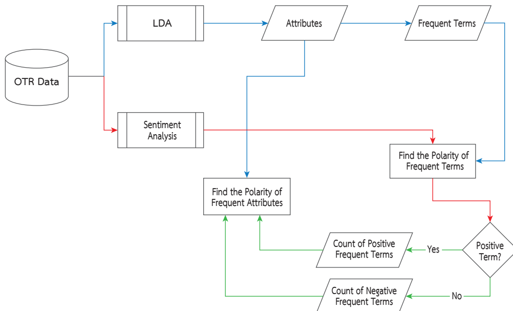
Figure 3: The Overview of the Attribute Analysis
