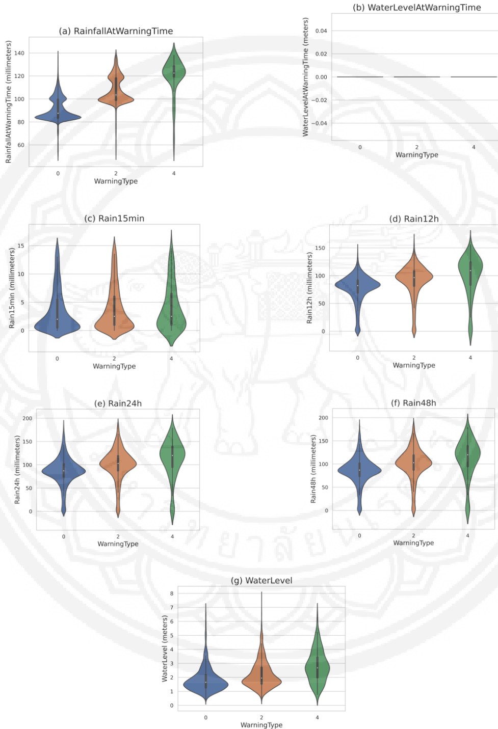
Figure 3 Violin plot for each feature
