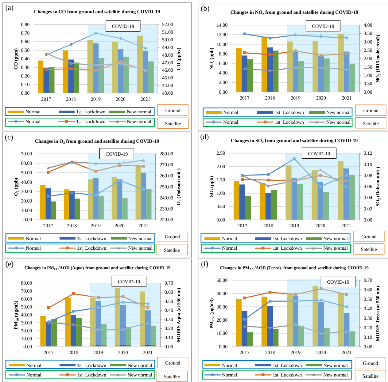
Figure 3 Trend of changes in air quality measurement data from the ground station and satellite during COVID-19 (2017-2021) (a-f).
