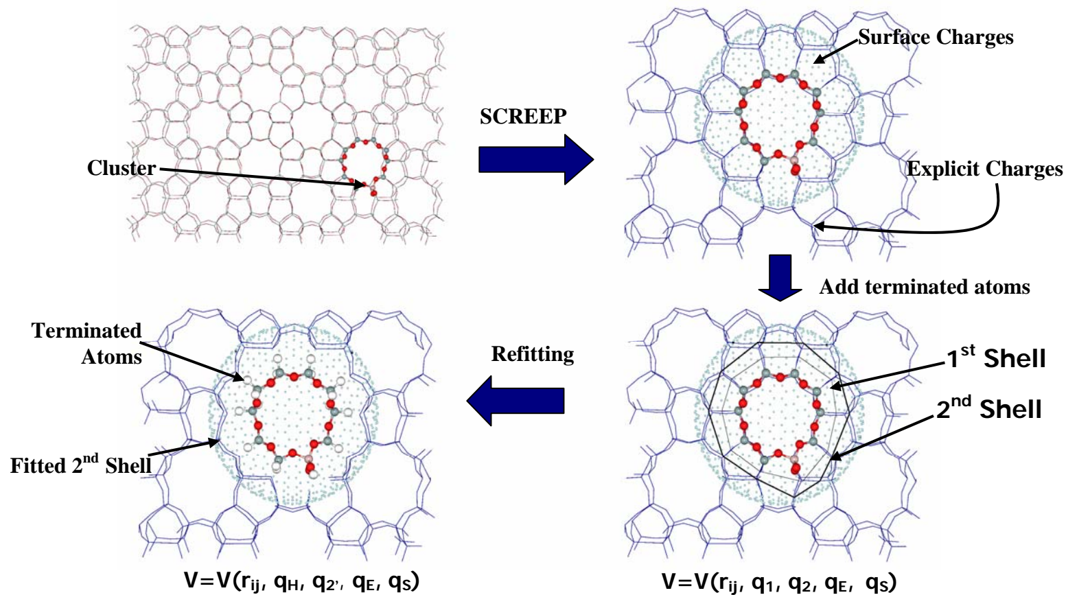
Appendix figure I Methodology for generating charges representing the zeolite framework by the SCREEP method
