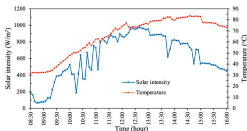
Fig. 5. Profiles of solar radiation intensity and temperature at different time in one day.
