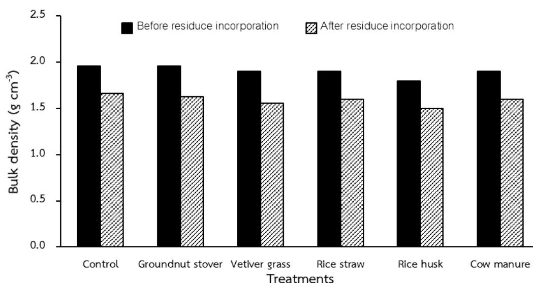
Figure 6 Bulk density at before and after organic residue incorporation
