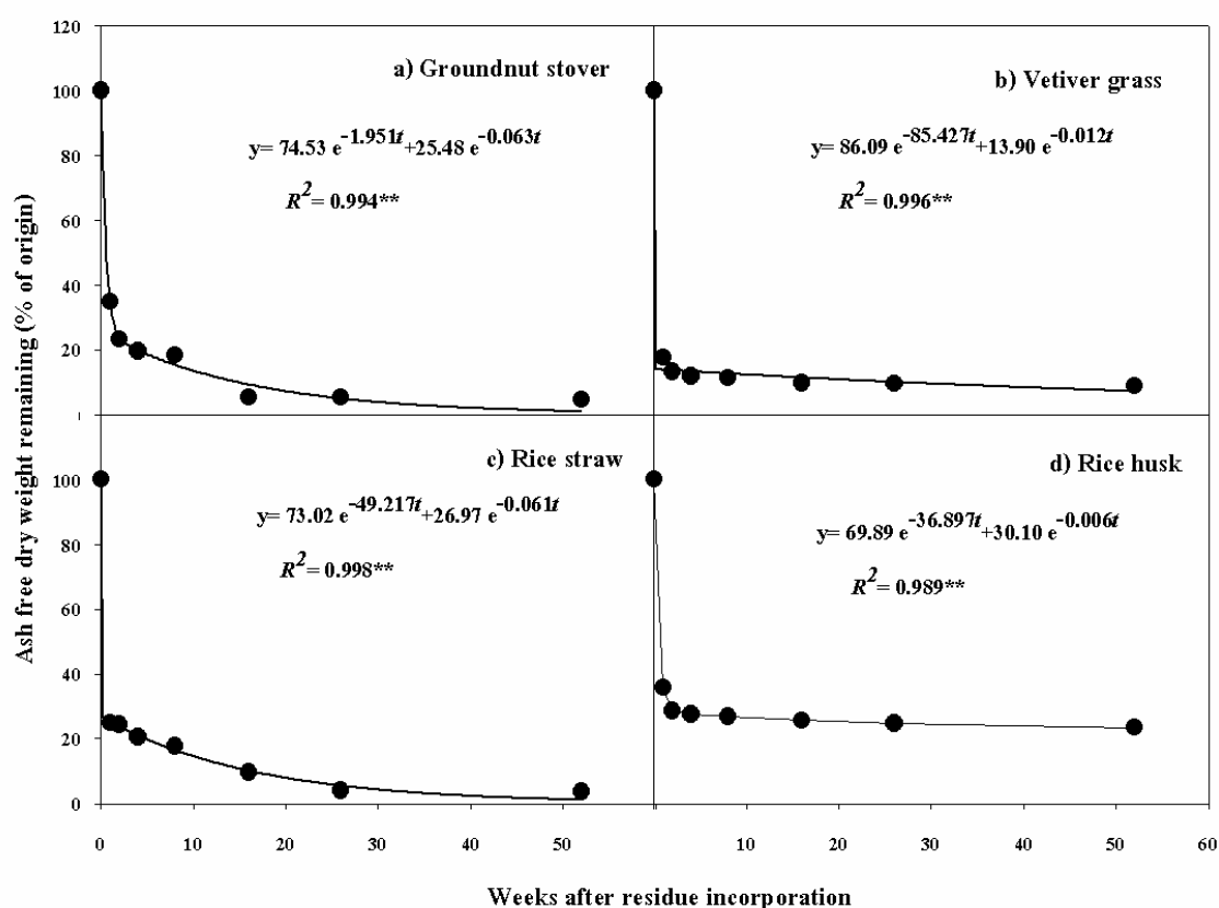
Figure 2 Dry weight remaining (% of origin) of different organic residue chemical composition after Incorporation
