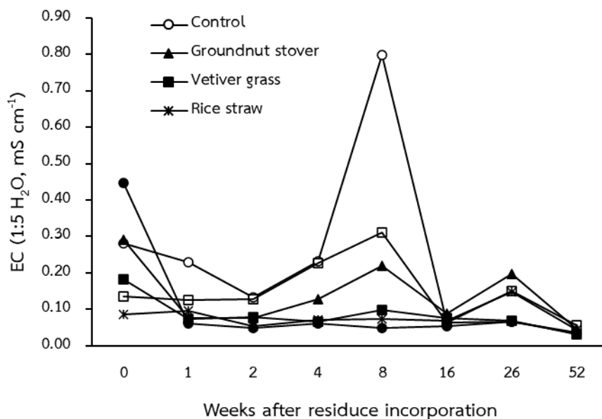
Figure 6 Electrical conductivity (1:5 H 2 O, mS cm -1 ) after organic residue incorporation
