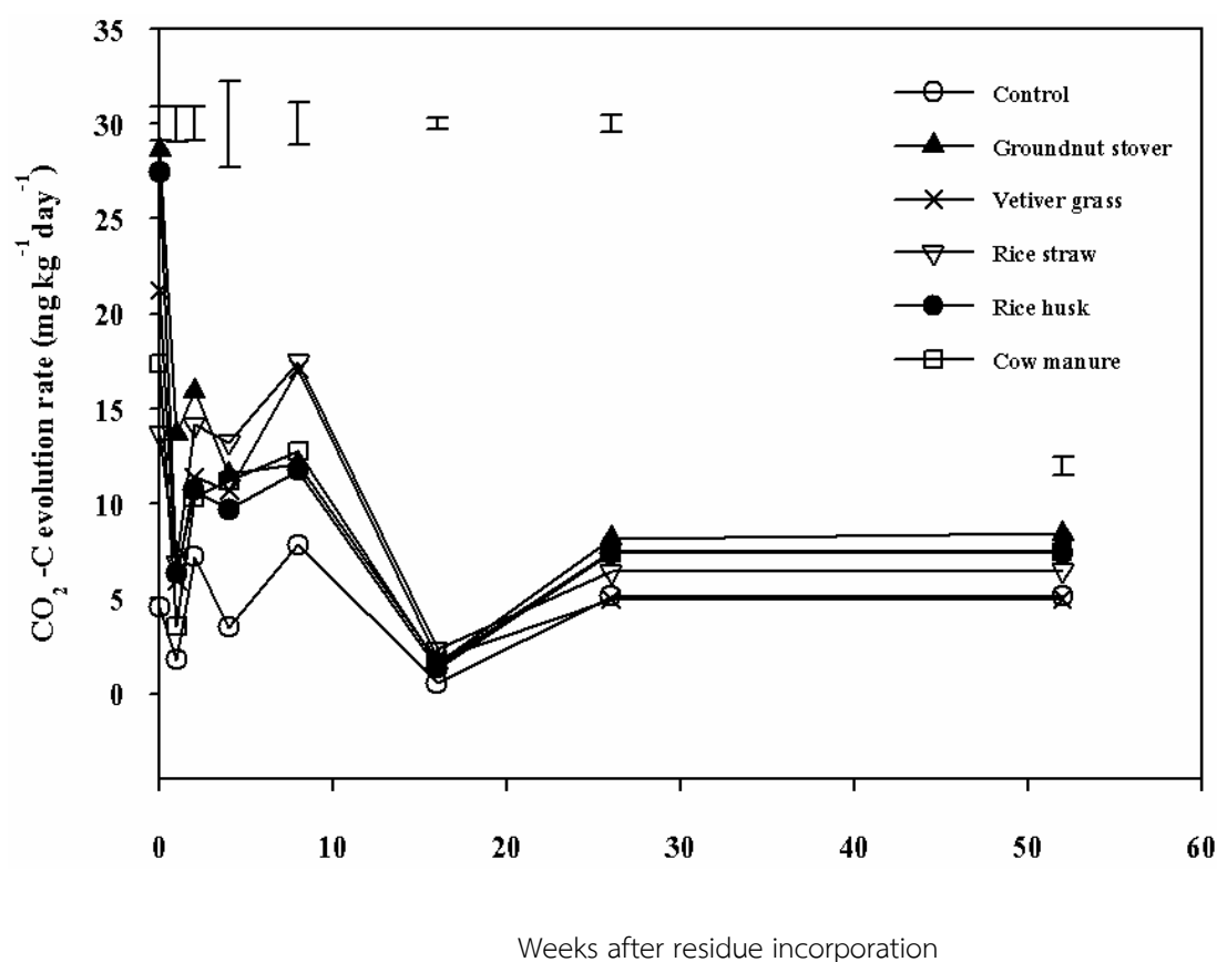
Figure 3 Carbon dioxide (CO 2 -C) evolution (mg kg -1 day -1 ) as affected by different organic residue incorporation
