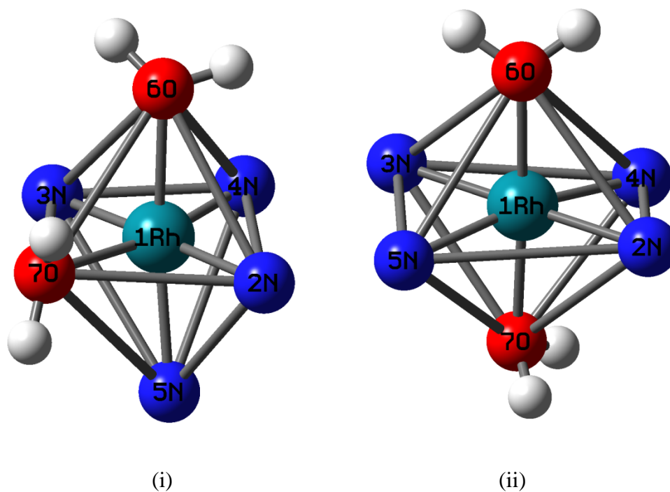
Figure 94 The geometry of coordinated bond between rhodium ion and donor atoms in (i) cis\text{-}[\text{Rh}(p\text{-TAA-n})_2(\text{H}_2\text{O})_2]^{3+} and (ii) trans\text{-}[\text{Rh}(p\text{-TAA-n})_2(\text{H}_2\text{O})_2]^{3+} .
