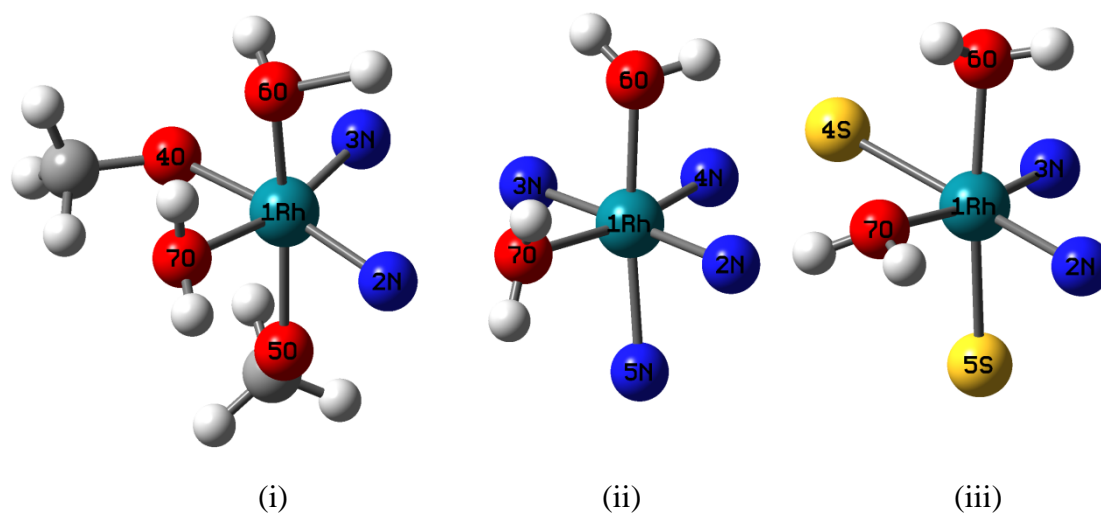
Figure 99 The coordination of different donor atoms to rhodium ion in (i) cis\text{-}[\text{Rh}(p\text{-TAA})_2(\text{H}_2\text{O})_2]^{3+} , (ii) cis\text{-}[\text{Rh}(p\text{-TAA-n})_2(\text{H}_2\text{O})_2]^{3+} and (iii) cis\text{-}[\text{Rh}(p\text{-TAA-s})_2(\text{H}_2\text{O})_2]^{3+} .
