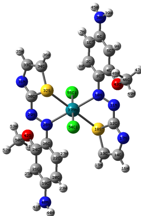
Figure 88 The optimized structure of trans\text{-}[\text{Rh}(p\text{-TAA-s})_2(\text{Cl})_2]^+ (GaussView 3.09).
