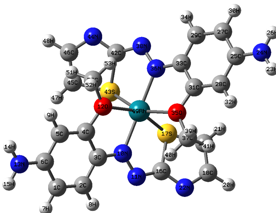
Figure 77 The optimized structure of [\text{Rh}(p\text{-TAA-s})_2]^{3+} (GaussView 3.09).
