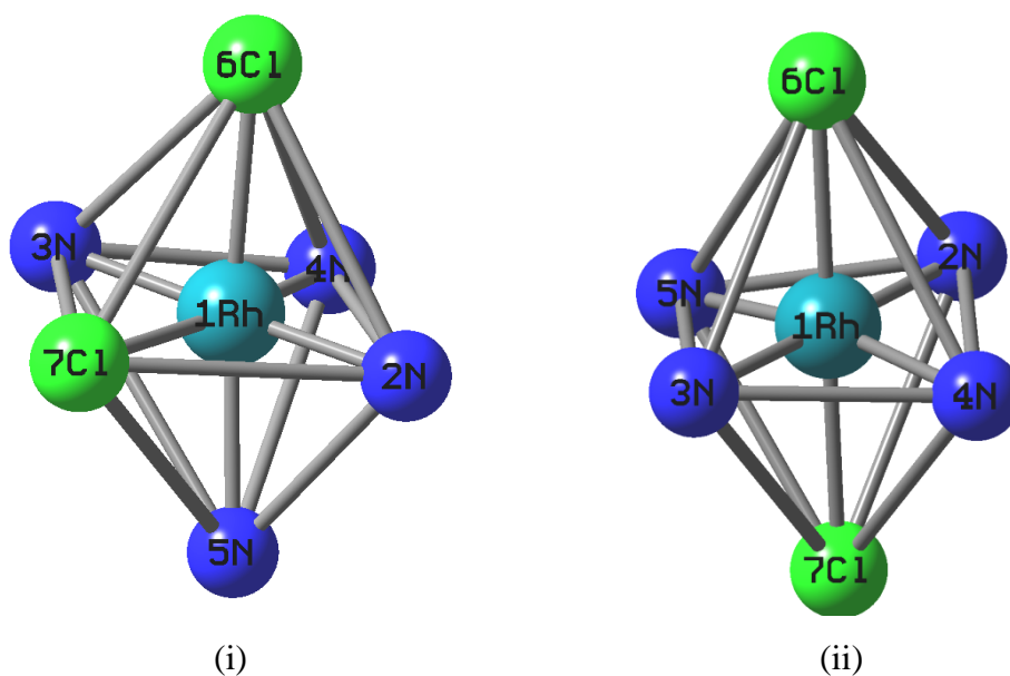
Figure 93 The geometry of coordinated bond between rhodium ion and donor atoms in (i) cis\text{-}[\text{Rh}(p\text{-TAA-n})_2(\text{Cl})_2]^+ and (ii) trans\text{-}[\text{Rh}(p\text{-TAA-n})_2(\text{Cl})_2]^+ .
