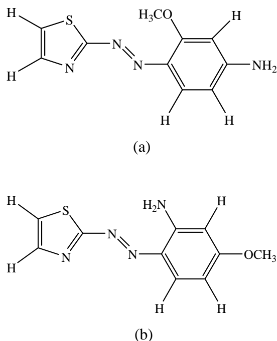
Figure 5 The structures of (a) 2-(2'-thiazolylazo)-5-aminoanisole ( p -amino TAA) and (b) 4-(2'-thiazolylazo)-3-aminoanisole ( o -amino TAA).
