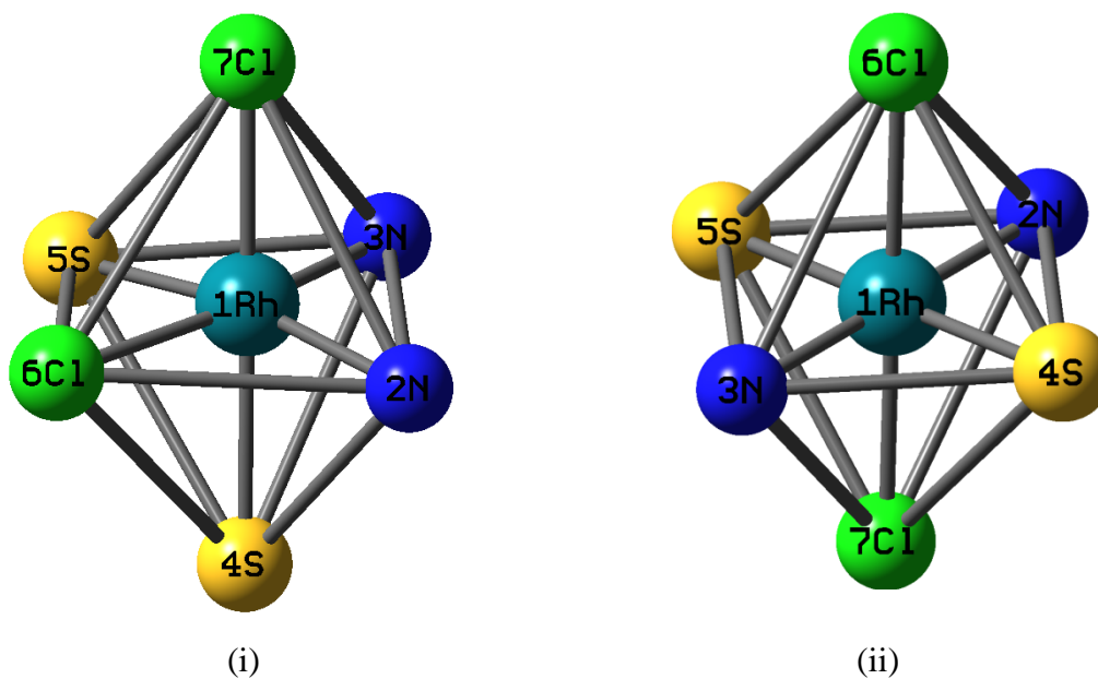
Figure 95 The geometry of coordinated bond between rhodium ion and donor atoms in (i) cis\text{-}[\text{Rh}(p\text{-TAA-s})_2(\text{Cl})_2]^+ and (ii) trans\text{-}[\text{Rh}(p\text{-TAA-s})_2(\text{Cl})_2]^+ .
