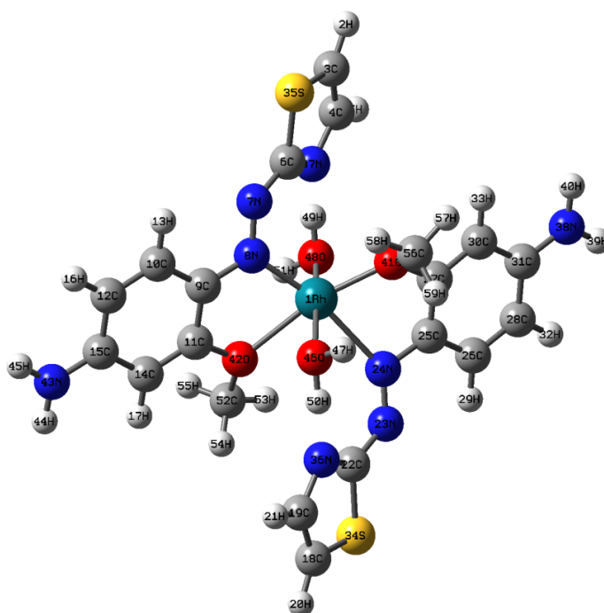
Figure 81 The optimized structure of trans\text{-}[\text{Rh}(p\text{-TAA})_2(\text{H}_2\text{O})_2]^{3+} (GaussView 3.09).
