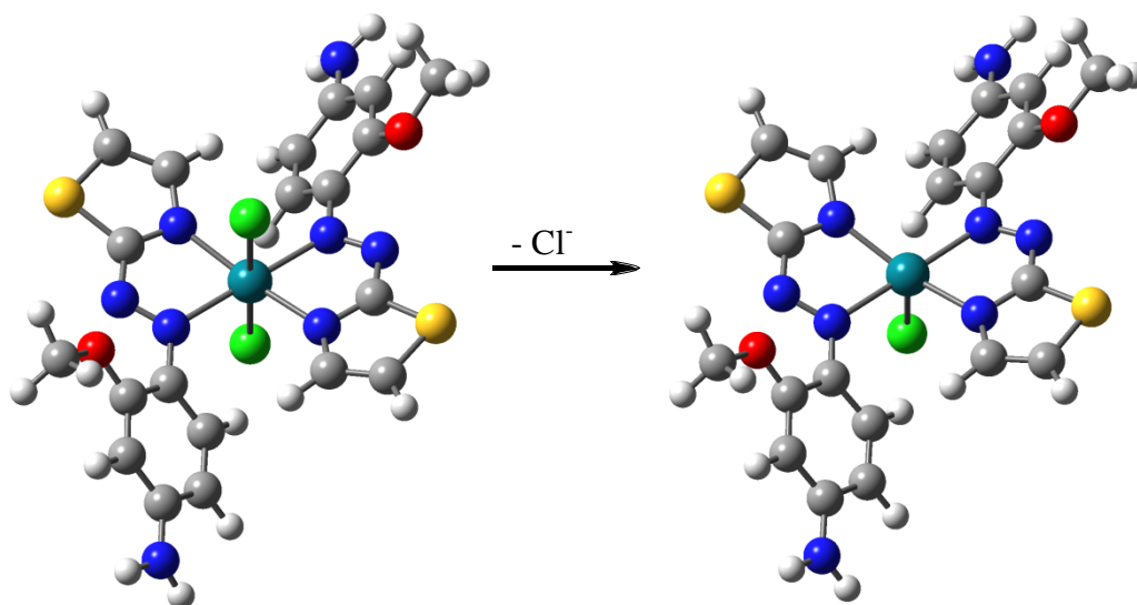
Figure 119 The five coordinated complex of trans\text{-}[\text{Rh}(p\text{-TAA-n})_2(\text{Cl})]^+ by removing chloride ion.
