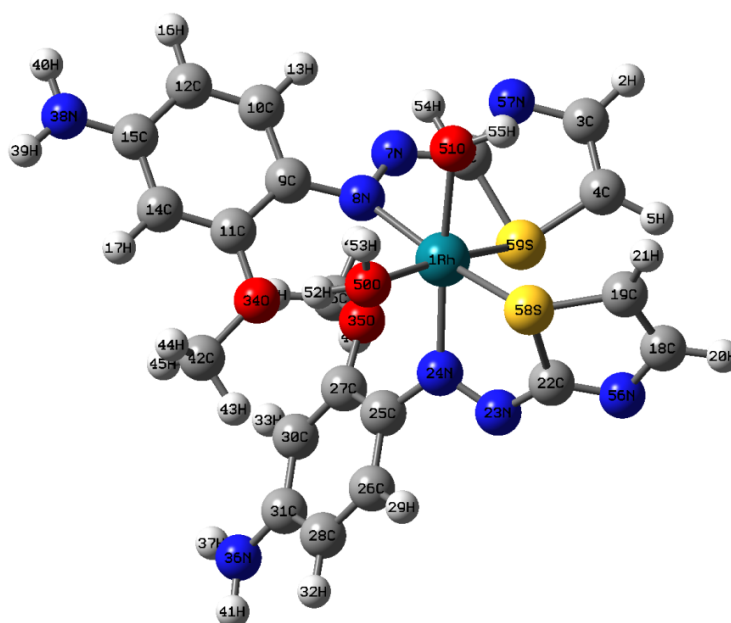
Figure 85 The optimized structure of cis\text{-}[\text{Rh}(p\text{-TAA-s})_2(\text{H}_2\text{O})_2]^{3+} (GaussView 3.09).
