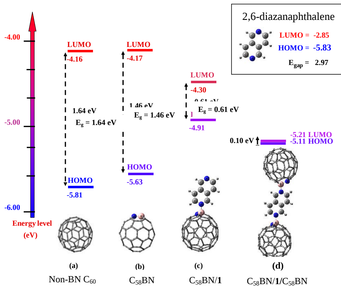
Figure 19 HOMO and LUMO orbital energies and energy gap of isolated 2,6-diazanaphthalene (1) and C 58 BN/1/C 58 BN complex
