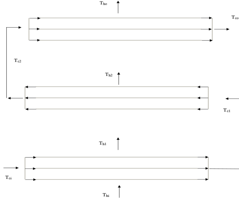
Figure 10: 3-pass cross flow heat exchanger
