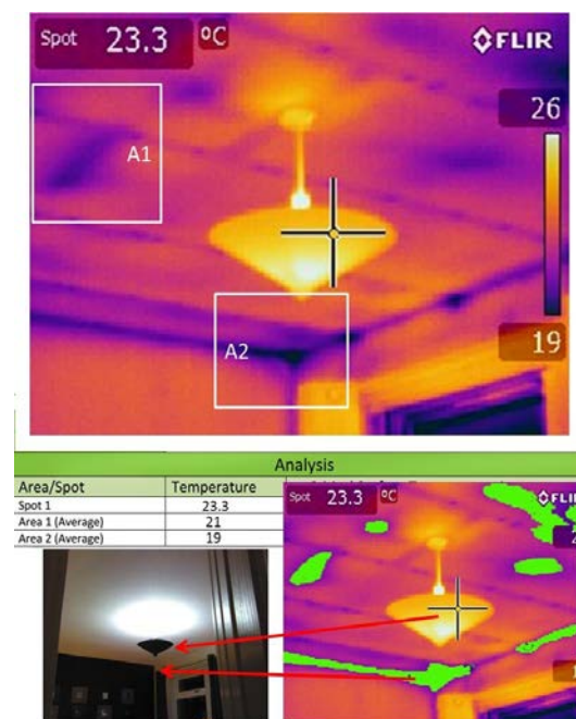
Figure 10: Using thermography for the bedroom
