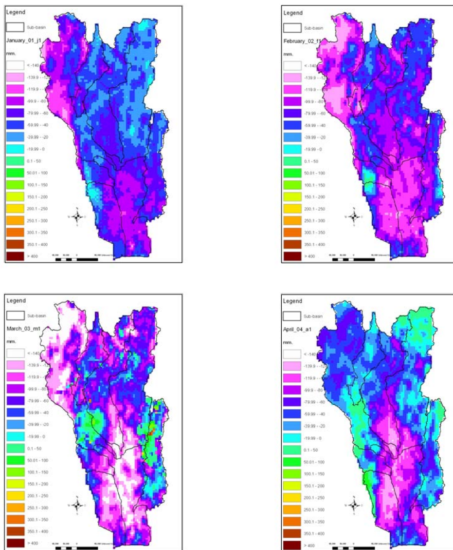
Figure 30 Spatial distribution of irrigation requirement from January to December
