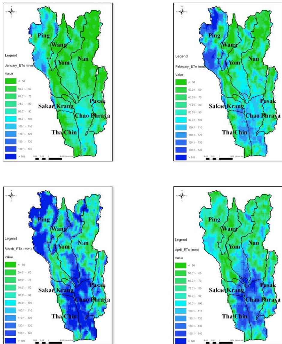
Figure 19 Spatial reference evapotranspiration from January to December
