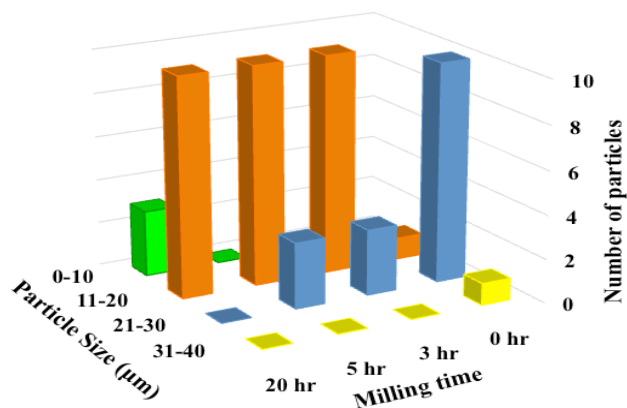
Figure 2. Particle size distribution of the ball-milled samples with various ball milling time.
